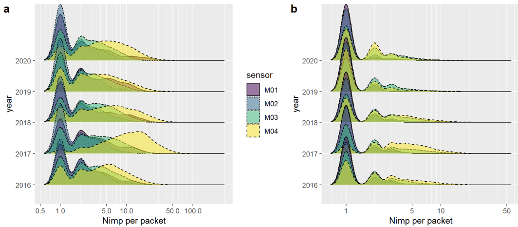
Figure S3: Erlenbach site. Combined no. of impulses (Nimp) of each sensor per packet by year. (a) Determined from the original data with a sampling rate of 20 kHz, (b) determined from the data down-sampled to 10 kHz. Transport intensities generally increase laterally in the measuring cross-section from the orographic left to right (in flow direction), implying that plate M04 observes higher transport intensities than plate M01.
