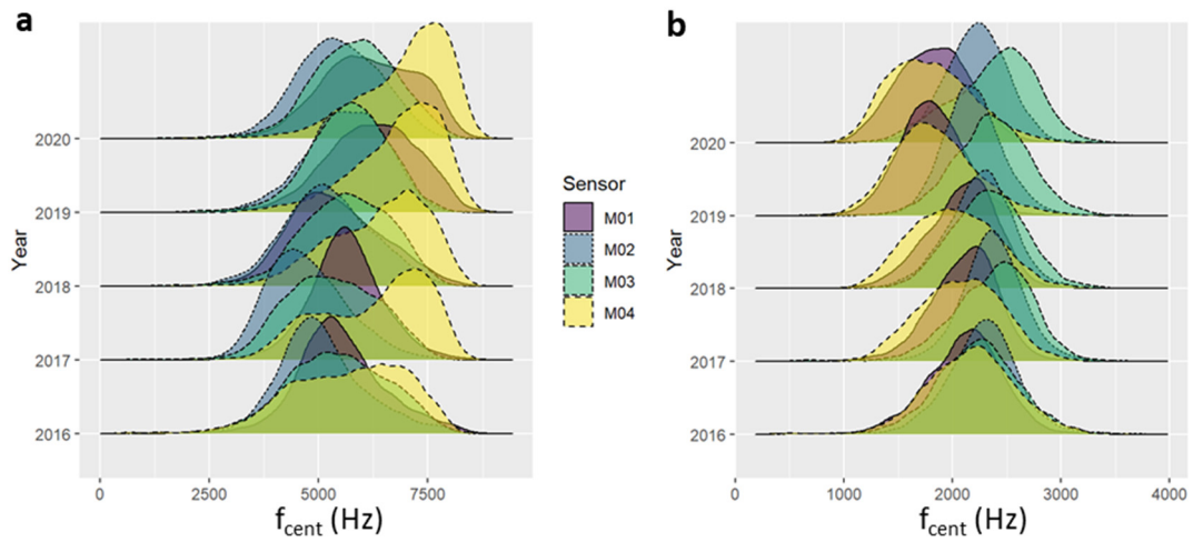
Figure S2: Erlenbach site. Centroid frequency of all packets by year. (a) Determined from the original data with a sampling rate of 20 kHz, (b) determined from the data down-sampled to 10 kHz.
