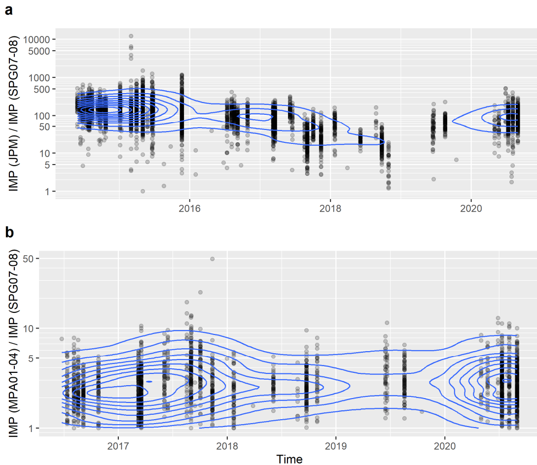
Figure S15: Erlenbach field site. Ratio of impulses of (a) JPM to SPG and (b) MPA to SPG per minute over multiple years. Time-steps with less than 10 GP impulses were removed for this plot. The blue lines are isolines of point density. (Note different time scales in panel a and panel b.)
