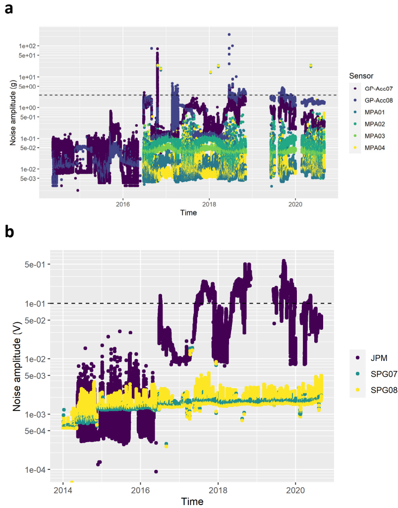
Figure S4: Background noise evolution over time. (a) MPA and GP-Acc at the Erlenbach. Accelerometer measurements before 20.06.2016 have been converted from V to g by multiplication with the conversion coefficient 100 g/V. (b) SPG and JPM at the Erlenbach.
