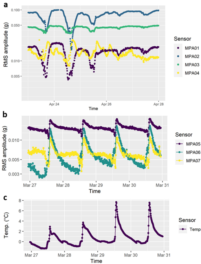
Figure S6: Daily cycles of the MPA noise level (i.e. root mean square RMS of amplitude) at (a) Erlenbach in April 2017 and (b) Avançon in March 2019, and (c) of water temperature in the Avançon stream in March 2019.
