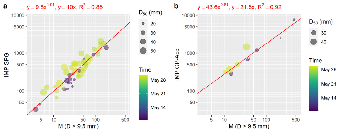
Figure S14: Albulu field site. Calibration relation in terms of number of impulses IMP vs. bedload mass M . (a) SPG impulses and (b) GP-Acc impulses plotted vs. direct bedload measurements. One GP-Acc calibration experiment was removed for this plot due to implausible signal presumably caused by sensor malfunctioning.
