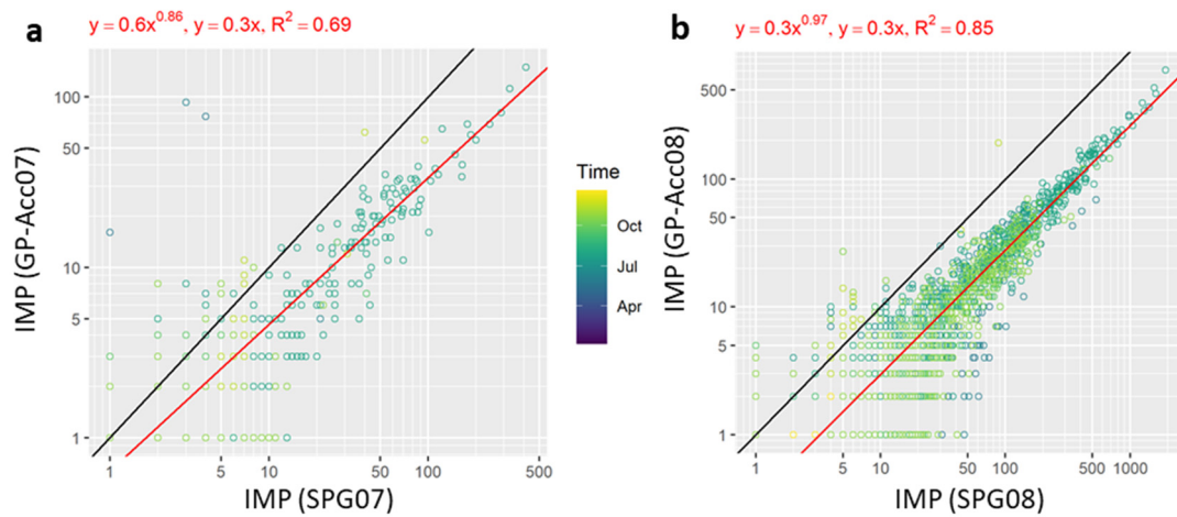
Figure S9: Erlenbach field site. Number of impulses IMP registered per minute with sensor GP-Acc vs. sensors GP-Geo (SPG), showing data for the year 2014 only. (a) Impacts on plate 07, on the left (in flow direction) of the channel center line, with generally weaker bedload transport; (b) Impacts on plate 08, on the right of the channel center line, with generally stronger bedload transport. All the time steps for which either of the two sensors registered zero impulses were removed for plotting. Black line: 1:1-line, red line: power-law regression. For the fit of the power-law, only IMP (SPG) > 50 and IMP (GP-Acc) > 10 were used. Note that the level of the IMP values of the two systems here cannot be compared to those in Figure 5 of the paper (where the Acc sensor has about 3 times more impulses than the Geo sensor). For the year 2014, the Acc Sensor was recorded in units of [V], and the IMP values per minute for the Acc Sensor were based on a threshold level of 0.1 [V], see also Table 2 of the paper, resulting in a low impulse count. For the calibration data (also for the period before June 2016) raw data were available, allowing to use a consistent threshold of 2.5 [g], as also used for the minute values in the period after Jun 2016.
