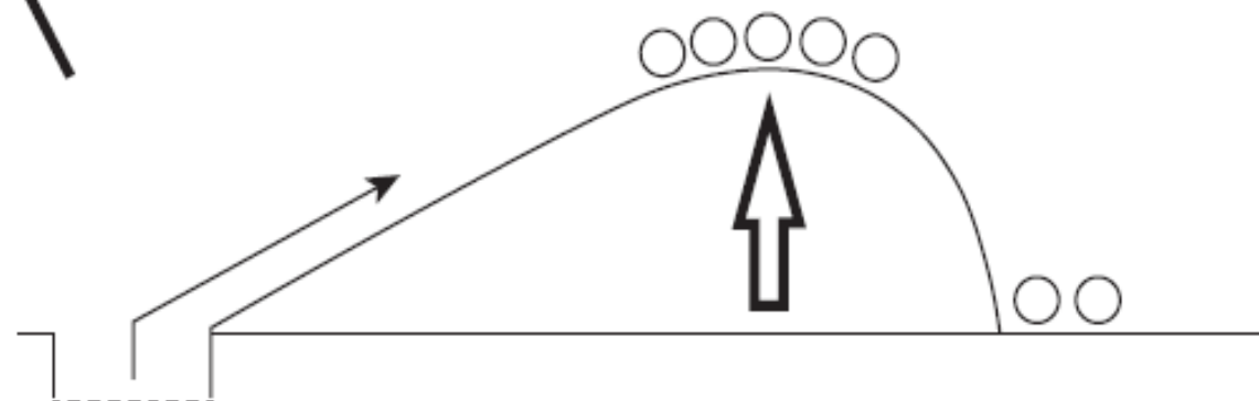
(e) Sediment redistribution and lower soil resistance triggers burrowing activity
