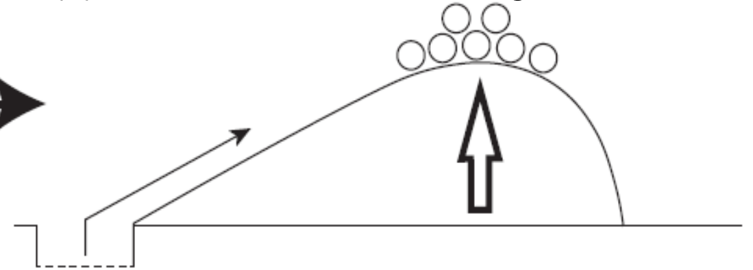
(b) Effect of animal burrowing
