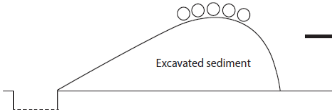
(a) Initial surface
