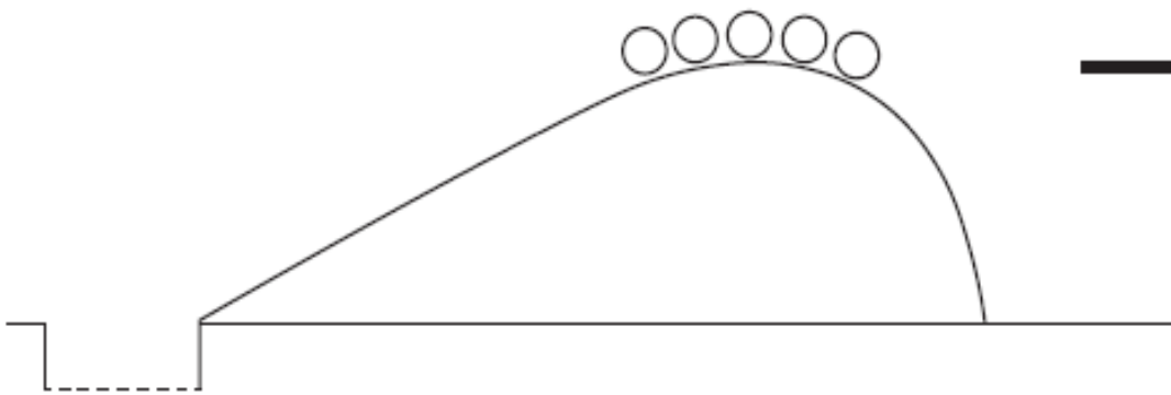
(c) Initial surface
