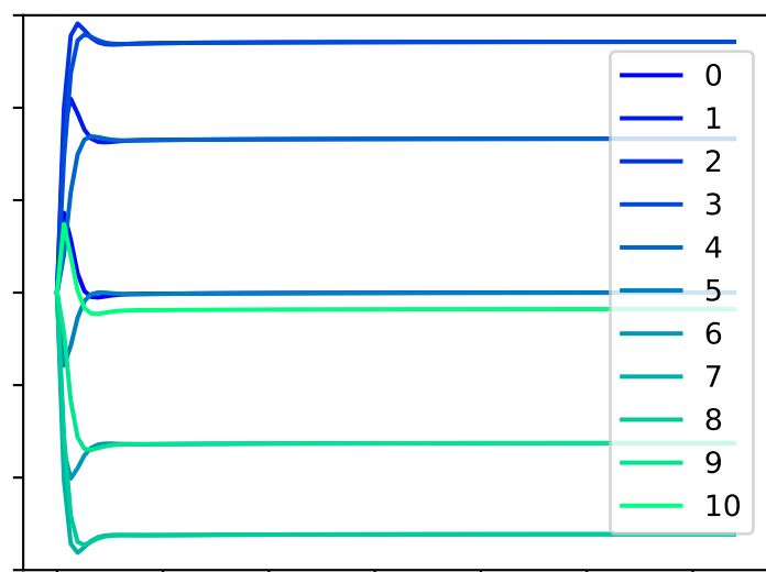
(e) TL model with P = \tau/10
