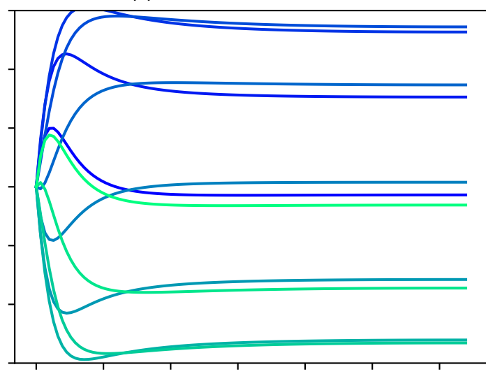
(g) TL model with P = \tau \times 10
