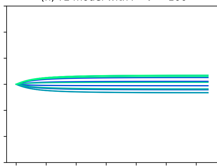
(h) TL model with P = \tau \times 100
