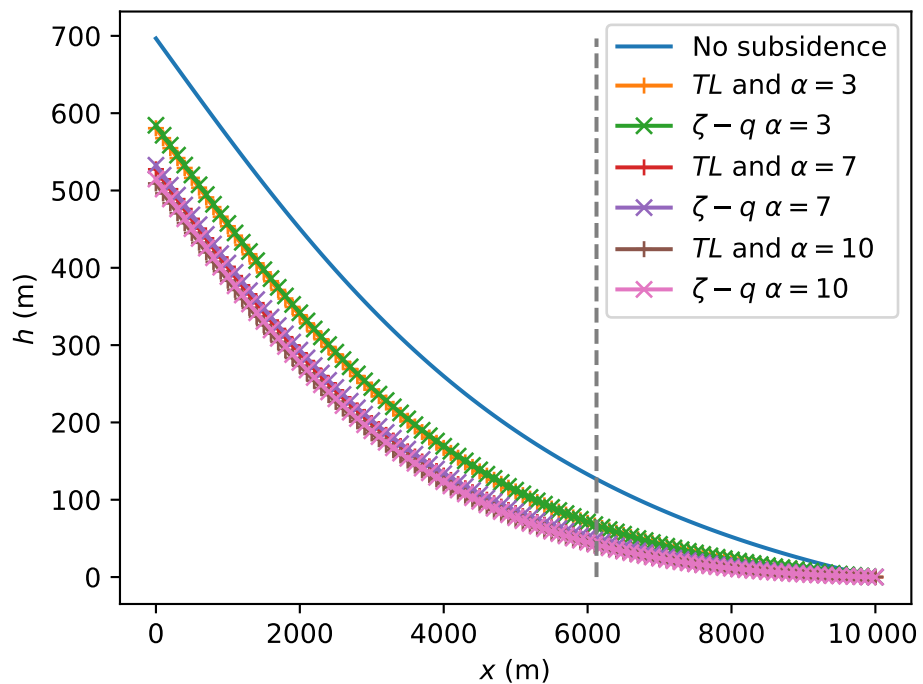
(d) Varying \alpha with s_0 = 0.001 m/yr and L \approx L_0
