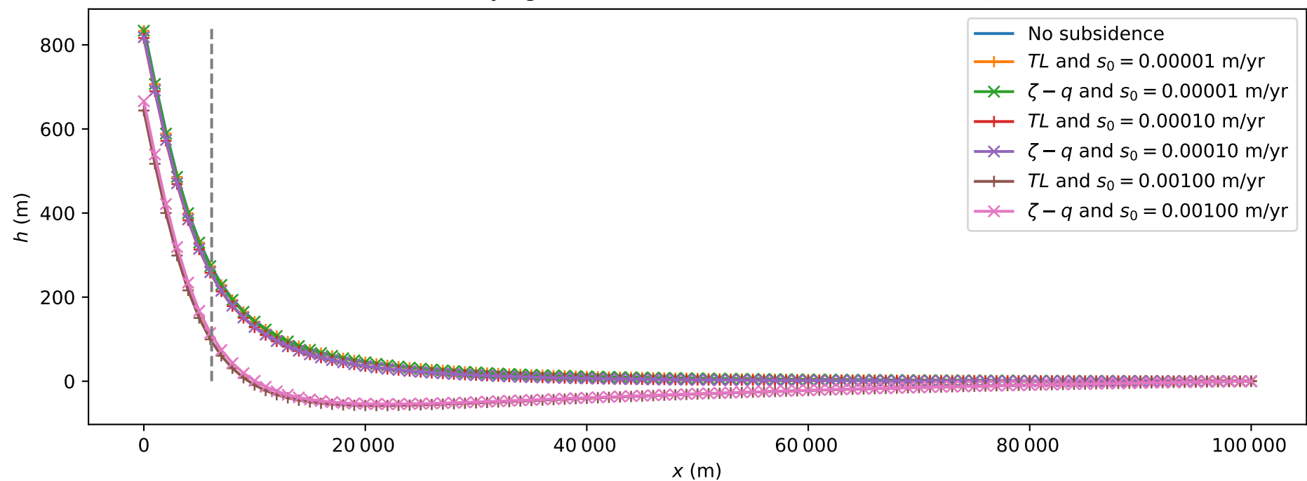
(a) Varying subsidence rate with \alpha = 7 and L \gg L_0
