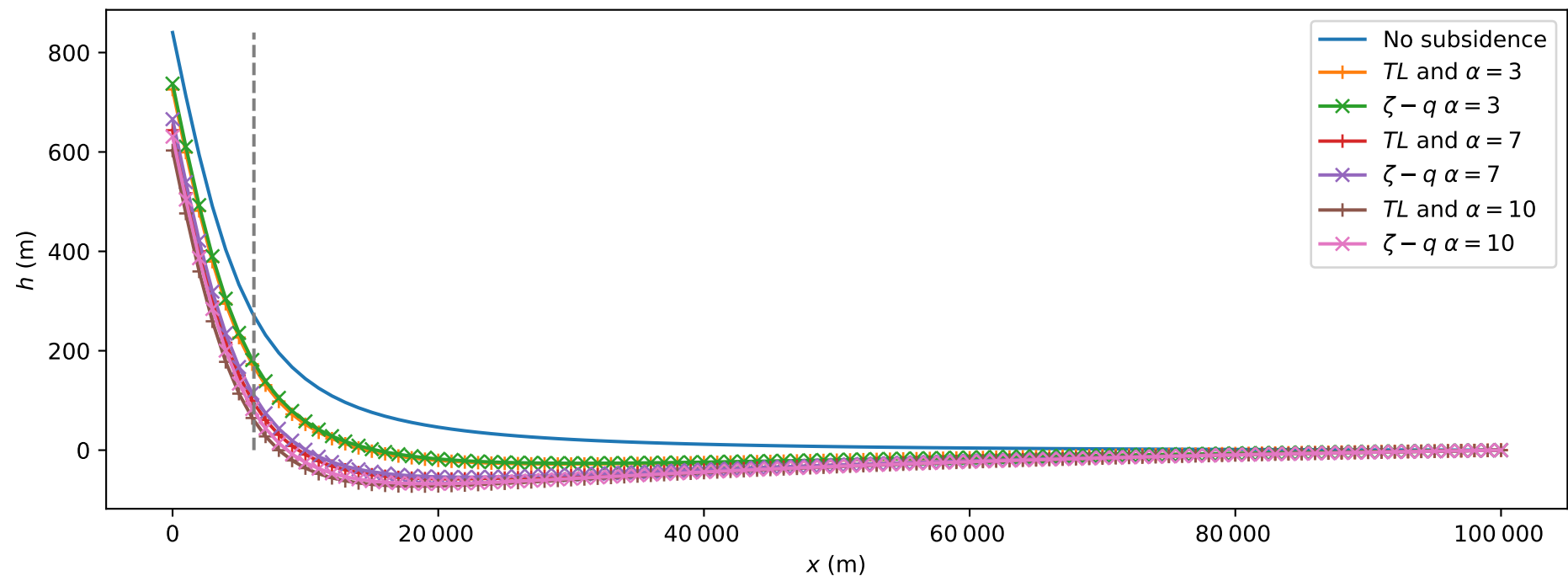
(b) Varying \alpha with s_0 = 0.001 m/yr and L \gg L_0
