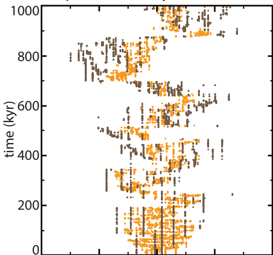
(c) erosion-only
