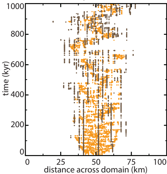
(c) erosion-only
