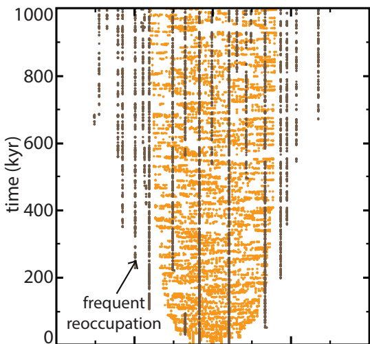
(b) deposition-only
