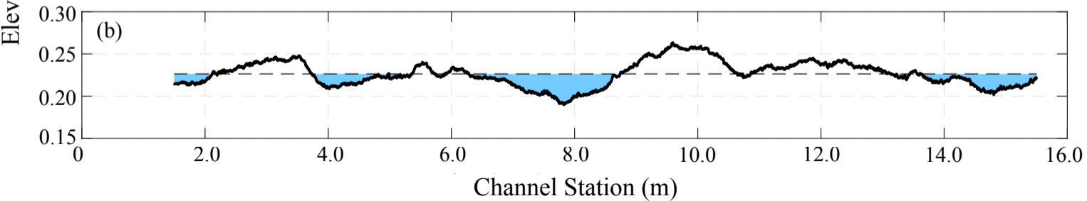
PRE4 Phase 2 Raw Profile at t1752 minutes
