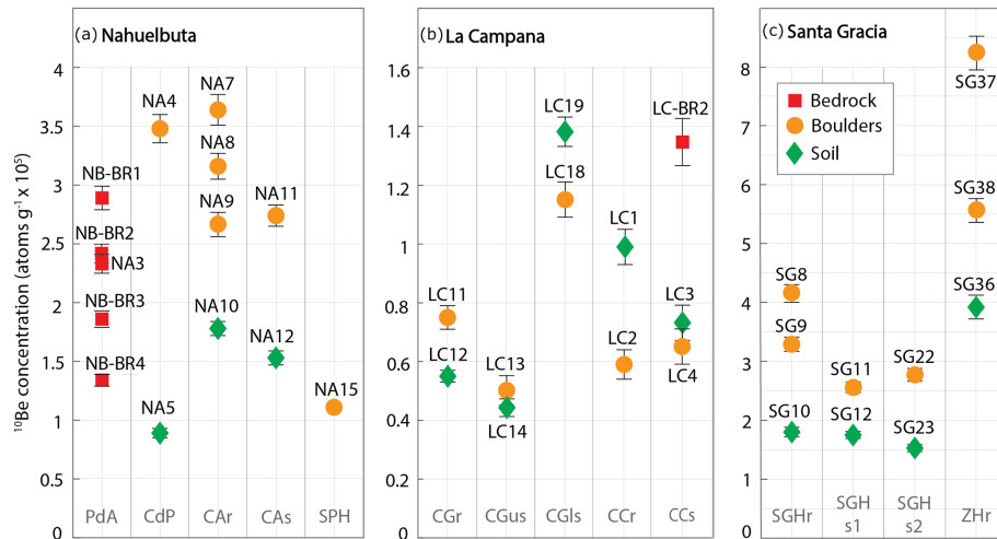
Figure 4. Measured ^{10}\text{Be} concentrations normalized to reference production rate at sea level high latitude for (a) Nahuelbuta, (b) La Campana, and (c) Santa Gracia; note the different scales of y axes. The x axes are not numerical but rather show the sampling locations, also reported in Table 1. Labels next to data points provide sample IDs, also reported in Table 1. Gray labels at the bottom of panels are the sample locations. PdA: Piedra de Aguila, CdP: Casa de Piedas, CAR: Cerro Anay ridge, CAs: Cerro Anay slope, SPH: Soil Pit Hill, CGr: Cerro Guanaco ridge, CGus: Cerro Guanaco upper slope, CGls: Cerro Guanaco lower slope, CCr: Cerro Cabra ridge, CCs: Cerro Cabra slope, SGHr: Santa Gracia Hill ridge, SGHs1: Santa Gracia Hill slope 1, SGHs2: Santa Gracia Hill slope 2, ZHr: Zebra Hill ridge.
