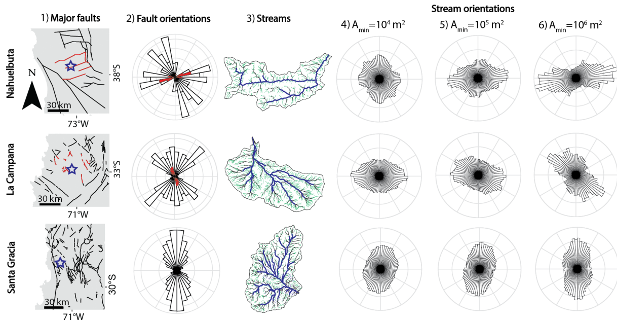
Figure 7. Rose diagram plots and maps showing fault and stream orientations for Nahuelbuta (top row panels), La Campana (middle row panels), and Santa Gracia (bottom row panels). For each field site, the columns show the following from left to right: (1) major faults digitized from a geological map (SERNAGEOMIN, 2003) within \sim 50 km (black) and \sim 25 km (red, NA and LC only) of the sampling site (blue star); (2) rose diagram of fault orientations from the maps in column 1, constructed using 100 m long, straight fault segments and 36 bins, with orientations of faults < 25 km from NA and LC in red; (3) a map of the studied catchments and the drainage network, with green, black, and blue streams indicating minimum upstream areas ( A_{\min} ) of 10^4 , 10^5 , and 10^6 m 2 , respectively, derived from 1 m resolution lidar DEMs (Kügler et al., 2022); (4–6) rose diagrams (72 bins) of stream orientations for different A_{\min} . All maps and rose diagrams are oriented with the top being north.
