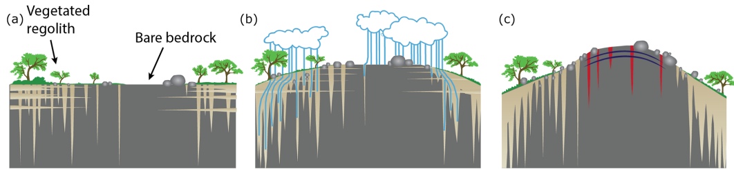
Figure 9. Schematic illustration showing the influence of bedrock fractures on landscape evolution. (a) Bedrock with different fracture densities is infiltrated to different degrees by rain and groundwater, which leads to differences in chemical weathering, soil formation, and vegetation growth, resulting in different hillslope sediment sizes. (b) Differential denudation between highly fractured and less fractured areas induces relief growth under slow but persistent uplift, which further promotes spatial gradients in chemical weathering, hillslope sediment size, and denudation. (c) Growing relief increases topographic stresses and the formation of new fractures (red) at topographically high positions (e.g., St. Clair et al., 2015) as well as unloading-related surface-parallel fractures (dark blue) (e.g., Martel, 2011), and steeper slopes allow for transportation of boulders, shown rolling down the slopes on either side.
