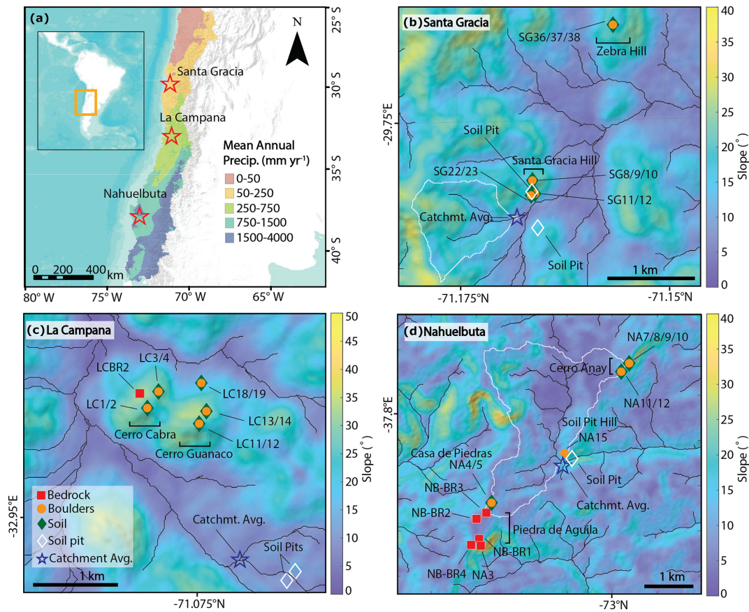
Figure 1. Field site locations and features. (a) Map of mean annual precipitation in central Chile, with field sites marked by red stars. Precipitation data from the CR2MET dataset, by the Center for Climate and Resilience Research (CR 2 ) (Boisier et al., 2018), provide an average for the time period 1979–2019. World Terrain Base map sources are Esri, USGS, and NOAA. B–D: slope and hillshade maps from 12.5 m ALOS PALSAR digital elevation models of (b) Santa Gracia (SG; Alaska Satellite Facility Distributed Active Archive Center, 2011b), (c) La Campana (LC; Alaska Satellite Facility Distributed Active Archive Center, 2019), and (d) Nahuelbuta (NA; Alaska Satellite Facility Distributed Active Archive Center, 2011a). Sample locations and sample names are shown, with symbol shape and color indicating the sample type (see legend in c). White outlines delineate the catchments from which the catchment average sample (star) was taken (the catchment from La Campana does not fit within the bounds of the map and is therefore not shown). Black lines indicate streams. Soil pit sample data are from Schaller et al. (2018), and catchment average sample data are from van Dongen et al. (2019).
