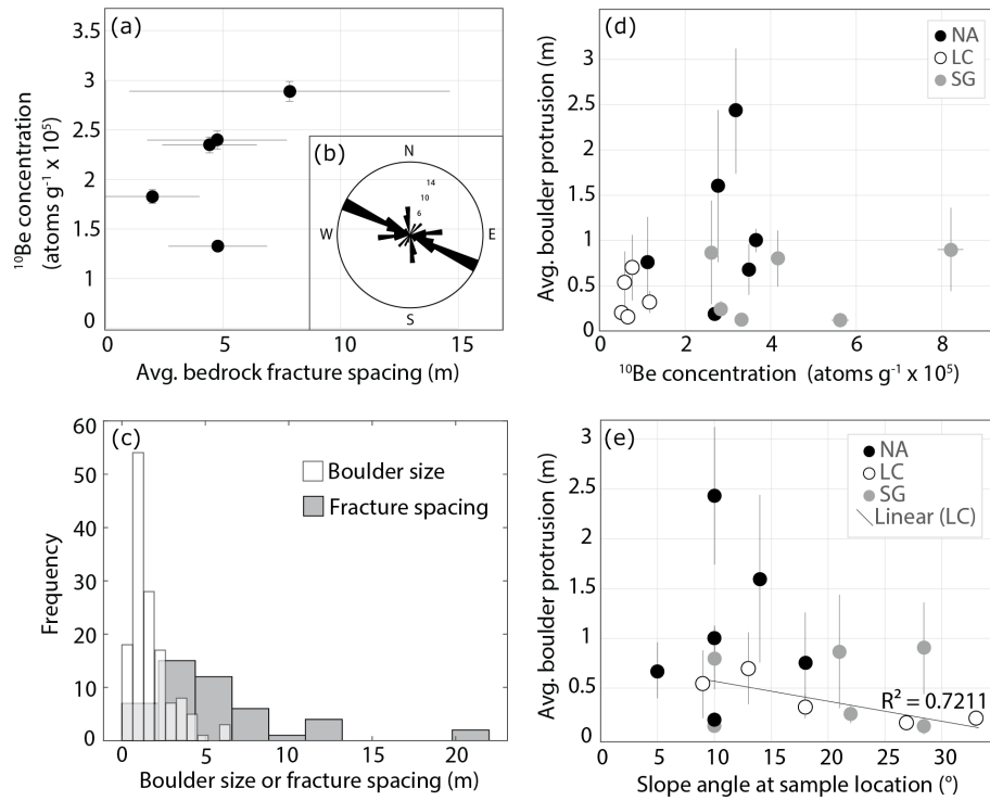
Figure 5. (a) Average bedrock fracture spacing (NA only), plotted against measured ^{10}\text{Be} concentrations normalized to the reference production rate at sea level high latitude. Error bars represent the standard deviation of all fracture spacing measurements for each location. (b) Rose diagram showing bedrock fracture orientations measured in the field in NA (same fractures as panel a). (c) Measurements of individual fracture spacing and individual boulder sizes, with boulder size being the average of the x and y axes of each boulder and the z axis the protrusion height. (d) Average boulder protrusion height plotted against measured ^{10}\text{Be} concentrations normalized to the reference production rate at sea level high latitude for each field site. Error bars represent the standard deviation of all boulder protrusion height measurements for each location. (e) Average boulder protrusion height plotted against hillslope angle. A linear regression model is fit through LC data points.
