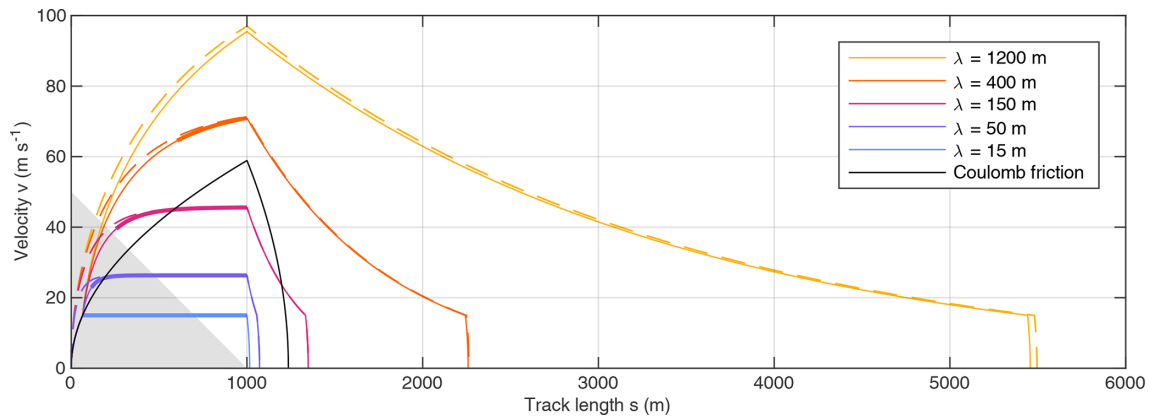
Figure 3. Phase space trajectories for \beta = 45^\circ , l = 1000 m, \mu = 0.75 , and v_c = 15 m s -1 . Solid lines start with Coulomb friction as long as v < v_c . Dashed lines correspond to a simplified scenario which immediately starts with flow instead of Coulomb friction. Thick line segments describe the range where flow is less efficient than Coulomb friction.
