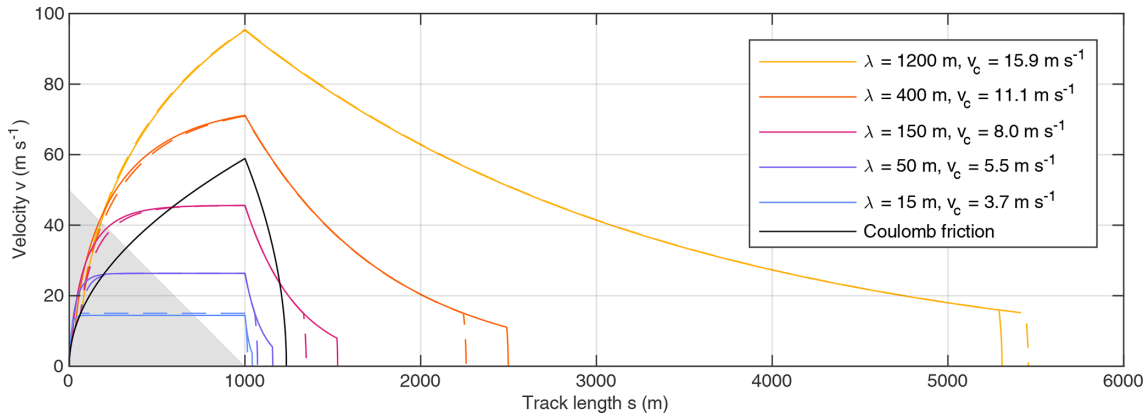
Figure 4. Phase space trajectories for \beta = 45^\circ , l = 1000 m, and \mu = 0.75 . Solid lines correspond to a given minimum RKE per mass (Eq. 18), while dashed lines describe the respective trajectories for v_c = 15 m s ^{-1} already shown in Fig. 3.
