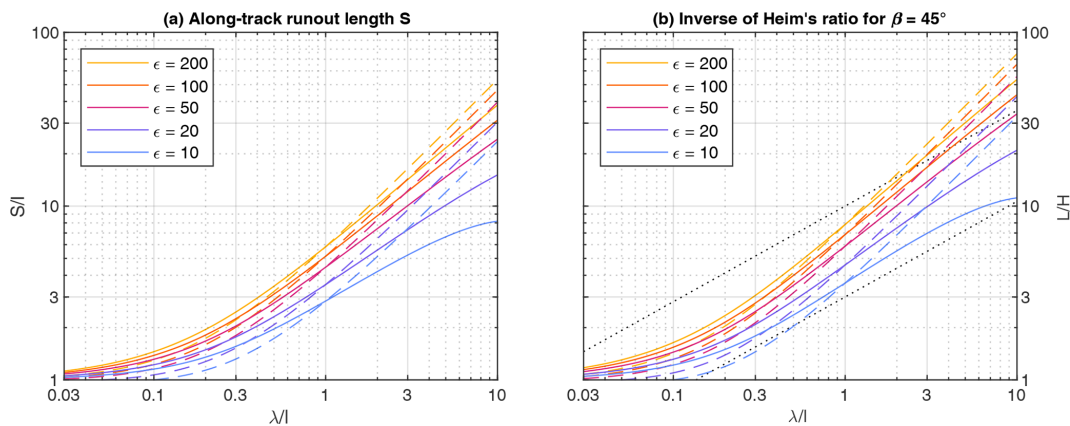
Figure 5. Runout length as a function of \lambda on the same topography (constant l and \beta for each curve). Dashed lines refer to the model with constant v_c (constant \epsilon along each curve). Solid lines refer to the RKE model, where \epsilon is the energy ratio for \lambda = l ( \epsilon(l, l) in Eq. 25). The dotted lines reflect the power law with an exponent \gamma = 0.55 expected from real rock avalanches.
