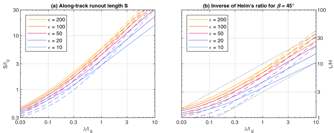
Figure 7. Runout length as a function of \lambda for slope length and height increasing with volume (Eq. 37 with \chi = 0.31 ). Dashed lines refer to the model with constant v_c and solid lines to the RKE model. The energy ratio in the legend refers to \lambda = l = l_0 ( \epsilon(l_0, l_0) in Eq. 38). The dotted lines reflect the power law with an exponent \gamma = 0.55 expected from real rock avalanches.
