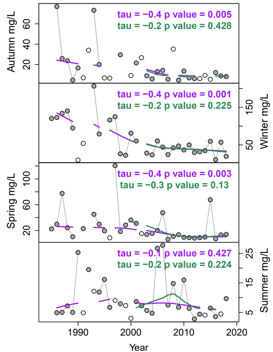
(c) Seasonal SSC
