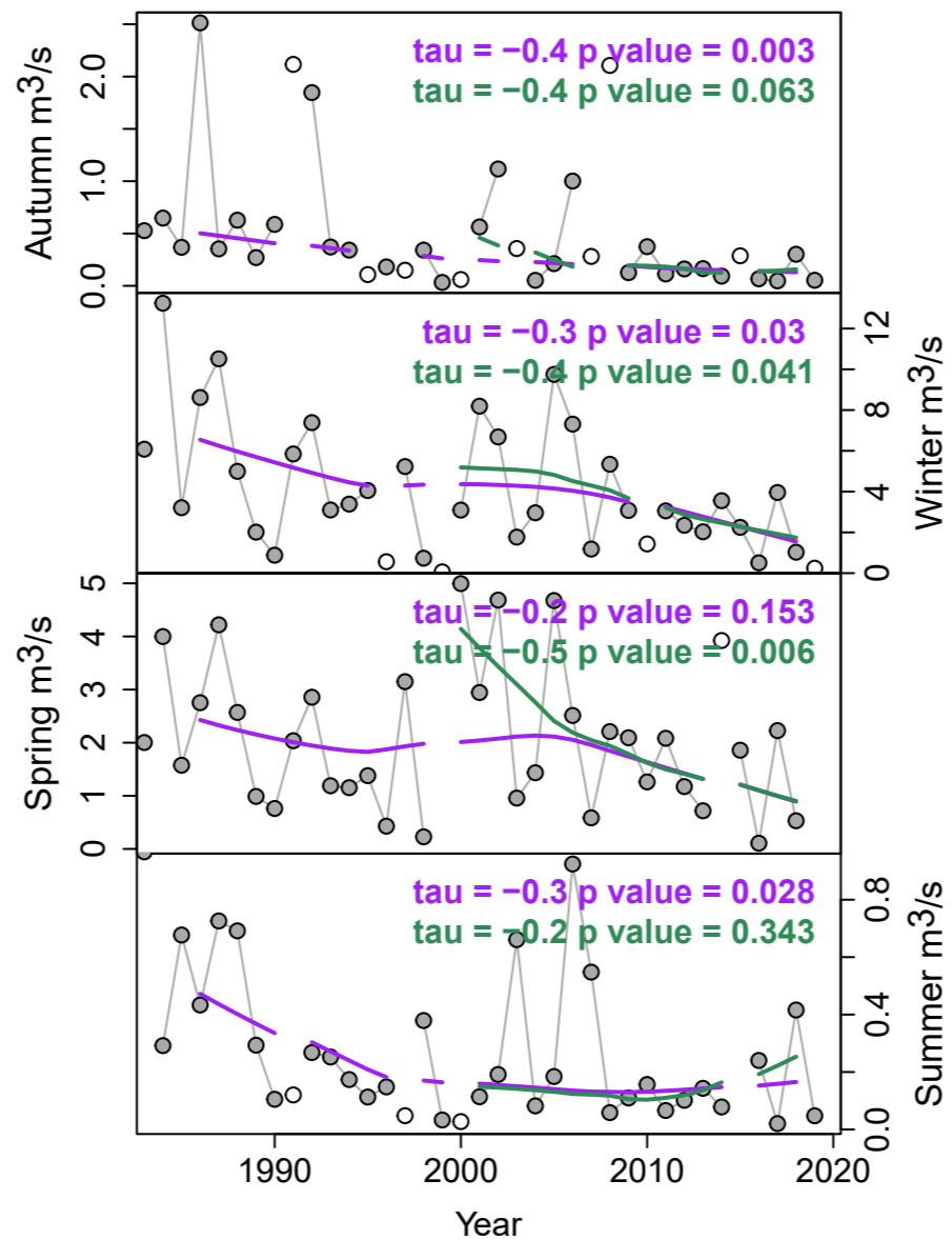
(b) Seasonal Baseflow
