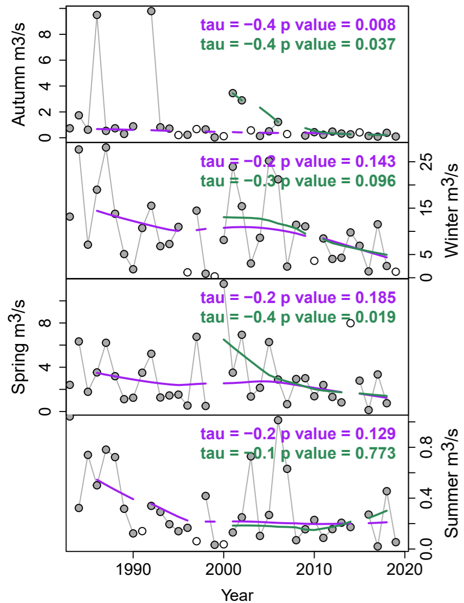
(a) Seasonal Streamflow
