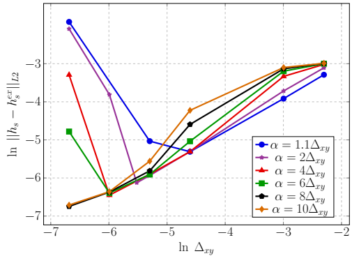
(b) kg = 1, kw = 50, rs = 2, ps = 0
