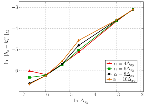
(a) kg = 1, kw = 50, rs = 3/2, ps = 1
