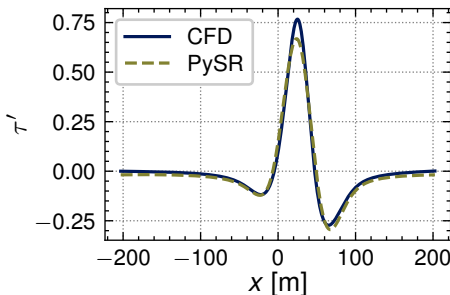
(c) Bump H/L = 0.2
