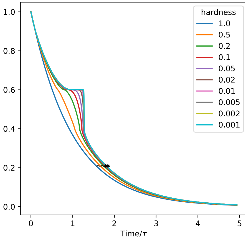
Position=0.5, Thickness=0.2
