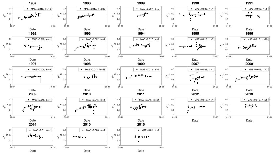
Figure S1. Best-fit model runs for every year on the record. “n” gives the number of models (i.e., parameter combinations) that minimize MAE and provide an equivalent best fit to the data. Annual best-fit parameters are also specified.
