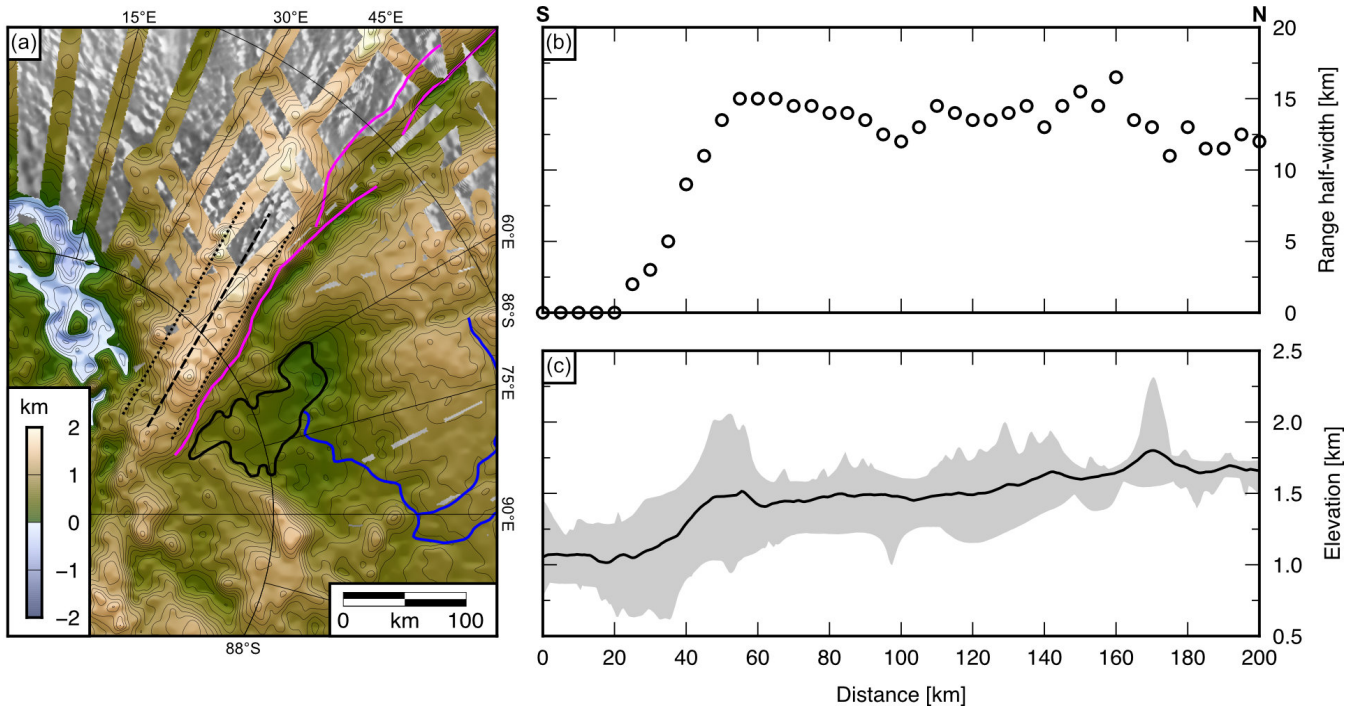
Figure S9: Growth of the Recovery Subglacial Highlands as a normal-faulted range. (a) Rebounded (ice-free) bed topography of the RSH; contour interval = 100 m (Paxman et al., 2022; Young et al., 2025). Annotations: purple = normal-faulted range front; black = smooth basin; blue = valleys. Dashed black lines mark the centre and edges of the topographic swath profile shown in panel c. (b) Range half-width as a function of distance along the RSH range front. Half-width was arbitrarily defined as half the distance between the 1500 m contour on either side of the range, measured at 5 km intervals along the profile. (c) Swath profile of rebounded bed elevation along the RSH. Solid line marks mean elevation and shaded field indicates the elevation range (minimum to maximum). The swath is oriented south-to-north and constitutes 20 parallel profiles within the region marked in panel a.
