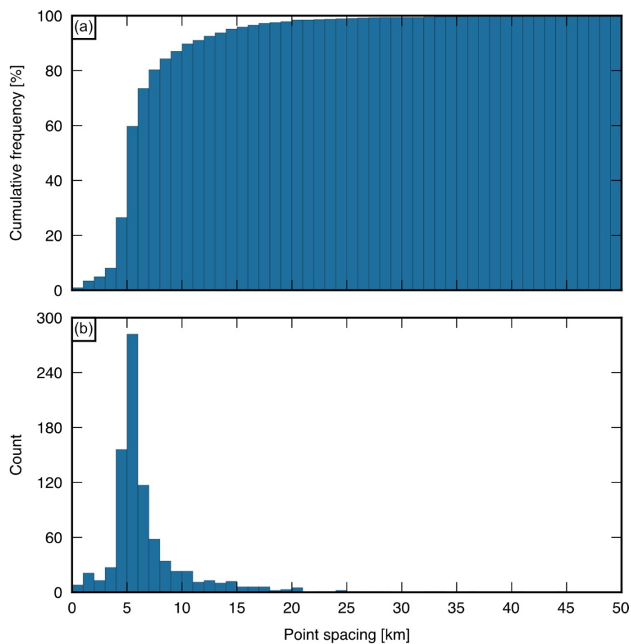
Figure S3: Frequency distribution of the spacing between adjacent RES measurement points along valley thalwegs. (a) Cumulative frequency distribution. (b) Histogram (by count; N = 852 ). The peak at 5–6 km corresponds to the average AGAP geophysical survey line spacing.
