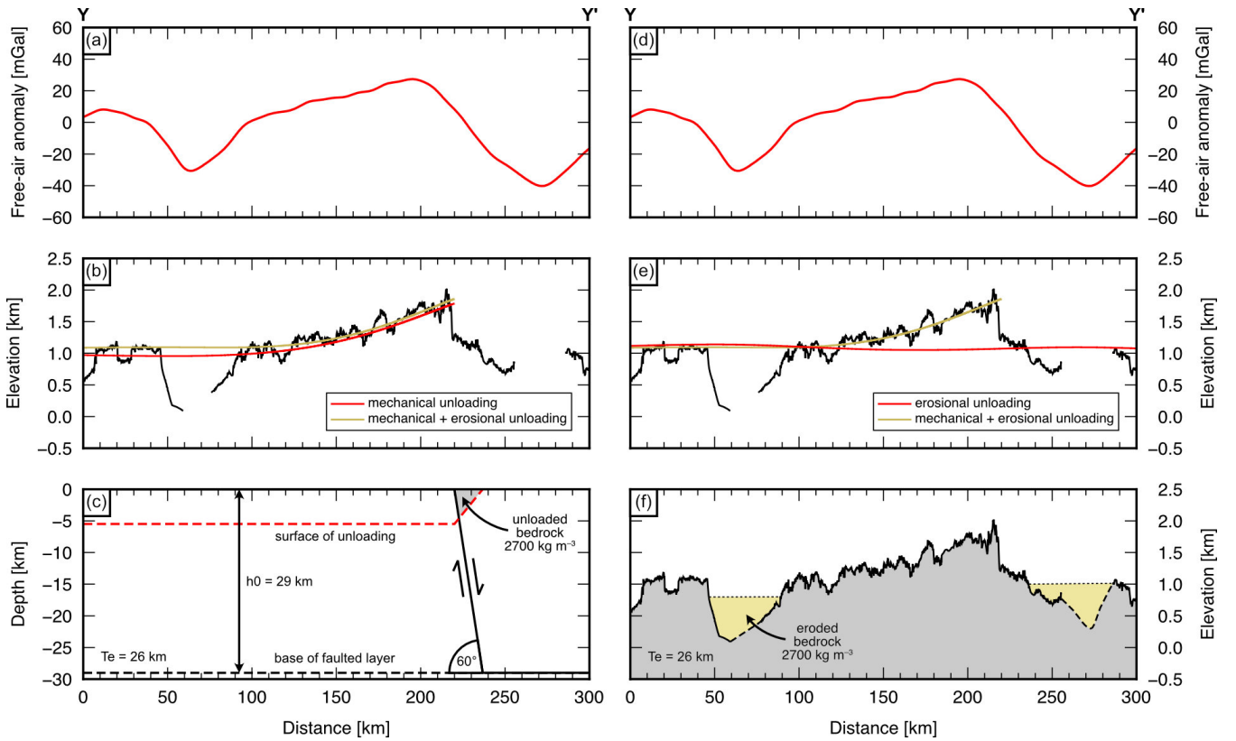
Figure S8: Flexural modelling of Recovery Subglacial Highlands uplift. (a) Free-air gravity anomaly along profile Y–Y' (location shown in Fig. 9 in the main manuscript) (MacGregor et al., 2021). (b) Modelled flexural uplift due to mechanical unloading. Black line is present-day bed elevation isostatically adjusted for the removal of the ice-sheet load (Paxman et al., 2022). Coloured lines show the flexural uplift triggered by mechanical unloading (red) and mechanical and erosional unloading combined (yellow) for a best-fitting combination of T_e = 26 km and h_0 = 29 km. (c) Fault model and unloading geometry. We assumed a single, purely normal fault with a typical dip of 60^\circ and a faulted layer thickness of h_0 . The grey wedge-shaped region represents the effective unloading experienced by the footwall block due to downward displacement of the hanging-wall block via slip on the fault. The region is bounded by Earth's surface, the fault, and the surface of unloading (elevation of the Moho under isostatic equilibrium in the absence of the crust) (Contreras-Reyes and Osses, 2010; Watts, 2023). (d) Free-air gravity anomaly (same as panel a). (e) As for panel b, except coloured lines show the flexural uplift triggered by erosional unloading (red) and mechanical and erosional unloading combined (yellow). (f) Erosion model and unloading geometry. We assumed erosion was focussed in the broad troughs either side of the highlands. The bed of the trough at \sim 270 profile-km was not imaged by RES; we used the observed gravity low at this point (panel d) to approximate the depth of the bed assuming a uniform bedrock density. Troughs were assumed to have been filled to a horizontal datum prior to excavation.
