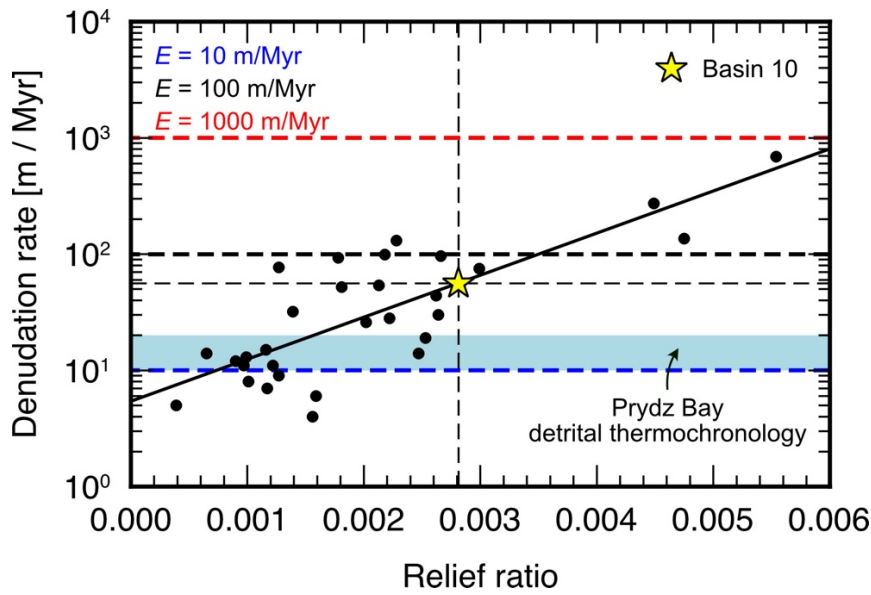
Figure S2: Global compilation of river basin denudation rates and relief ratios. Circles denote empirical data for individual river basins (Summerfield and Hulton, 1994); black trend line was calculated via linear least-squares regression ( R = 0.791 ). Blue, black, and red dashed lines mark denudation rates of 10, 100, and 1000 m/Myr, respectively, which were used for the three K scenarios in our models. Yellow star and dashed lines mark a relief ratio of 0.0028 (value for basin 10 in the Gamburtsevs), which corresponds to a denudation rate ( E ) of ~50 m/Myr. Blue horizontal bar denotes long-term catchment-averaged denudation rates (10–20 m/Myr) derived from thermochronological analysis of detrital sediments in Prydz Bay, East Antarctica (Thomson et al., 2013).
