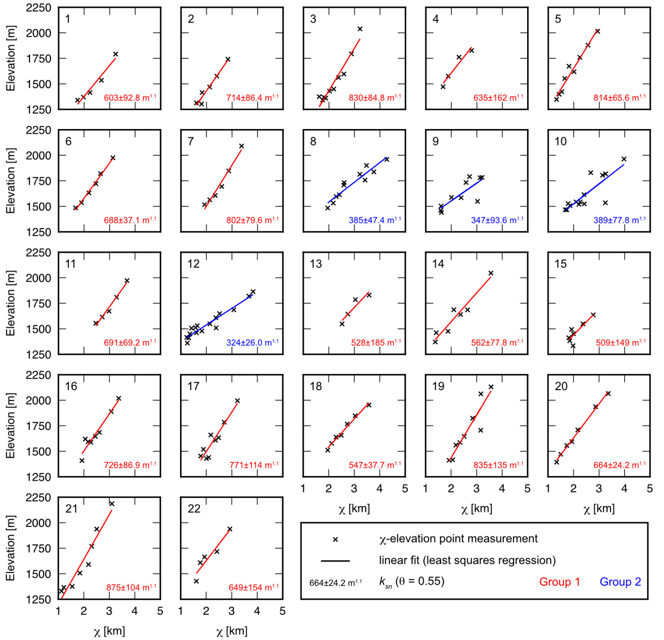
Figure S5: \chi analysis and estimation of k_{sn} for valley segments across the northern GSM. \chi -elevation plots are constructed for 22 valley segments, each assuming \theta_{\text{ref}} = 0.55 and A_0 = 10^6 \text{ m}^2 . Segment numbers are indicated in the upper left corners of the plots and correspond to the labels in Fig. 7 in the main manuscript. The values of k_{sn} are determined by linear least-squares regression, with uncertainties representing \pm 1 standard deviation.
