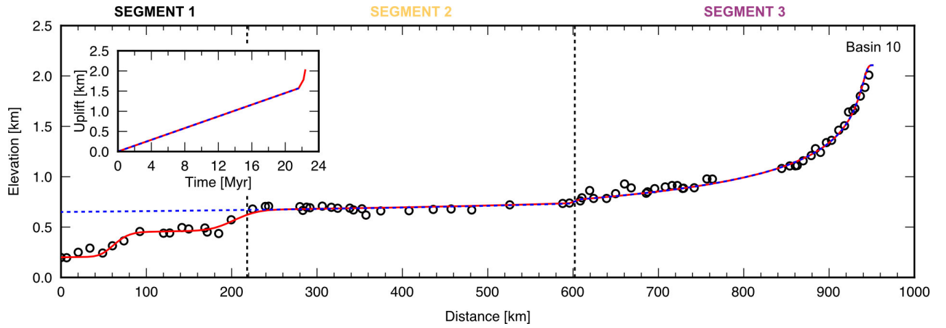
Figure S6: Stream power incision modelling with a temporally variable uplift rate. Comparison between modelled (coloured lines) and observed (circles) longitudinal profiles for basin 10. Vertical dashed lines mark boundaries between profile segments. The dashed blue line is the modelled longitudinal profile with a uniform U (equivalent to Fig. 8a in the main manuscript with identical SPIM parameters, E = 100 m/Myr, and a best-fitting model run time of 22 Myr). The modelled profiles for segments 2 and 3 have been combined, with a step-change in K at the boundary. The red line is a modelled longitudinal profile for a scenario where two pulses of uplift (or base-level fall) are included near the end of the model run, resulting in an improved fit with observations in segment 1 of the profile. Inset shows the corresponding uplift histories.
