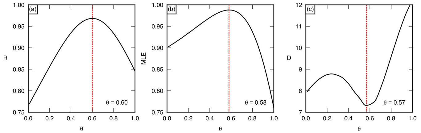
Figure S4: Comparison of methodologies used to identify the most appropriate concavity index ( \theta ) for drainage basin 10. (a) Correlation coefficient ( R ) between \chi and elevation for all trunk and tributary nodes, as determined via linear least-squares regression. (b) Maximum likelihood estimator (MLE) calculated from the residuals between the elevation of all tributary nodes and the linear regression of elevation on the trunk valley (i.e., a measure of the degree of collinearity between the tributaries and the trunk valley). (c) The disorder metric ( D ), a measure of how far tributaries depart from the trunk valley and among themselves in \chi -elevation space. Each metric is calculated as a function of \theta . Dashed red lines mark the 'best-fit' value of \theta for each plot, given by the maximum value of R and MLE, and the minimum value of D .
