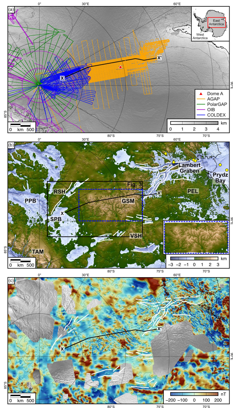
Figure 1. Regional setting of the Gamburtsev Subglacial Mountains. (a) Airborne radio-echo sounding surveys used in this study, overlain on hillshaded surface elevation from the Reference Elevation Model of Antarctica (contour interval = 1 km) (Howat et al., 2019). Thick black line marks the grounding line (MEASURE version 2). Inset shows the study area within East Antarctica. (b) Bed elevation relative to mean sea level from Bedmap3 (contour interval = 1 km) (Pritchard et al., 2025). Profile X–X' is displayed in Fig. 2; box shows the extent of Fig. 3. White lines mark the East Antarctic Rift System (Ferraccioli et al., 2011). Yellow circles mark offshore sediment core and onshore moraine locations where samples have been collected for detrital thermochronological analysis (Thomson et al., 2013). Abbreviations: GSM = Gamburtsev Subglacial Mountains; PEL = Princess Elizabeth Land; PPB = Pensacola-Pole Basin; RSH = Recovery Subglacial Highlands; SPB = South Pole Basin; TAM = Transantarctic Mountains; VSH = Vostok Subglacial Highlands. Inset shows a perspective image of the Gamburtsevs (covering the dashed blue area). The topography is viewed from an azimuth of 180° and an angle of 70°, with ~20× vertical exaggeration. (c) ADMAP-2B magnetic anomaly compilation (contour interval = 200 nT) (Eagles et al., 2024; Golynsky et al., 2018). Data gaps are filled by the RADARSAT RAMP AMM-1 SAR image mosaic version 2 (Jezek et al., 2013).
