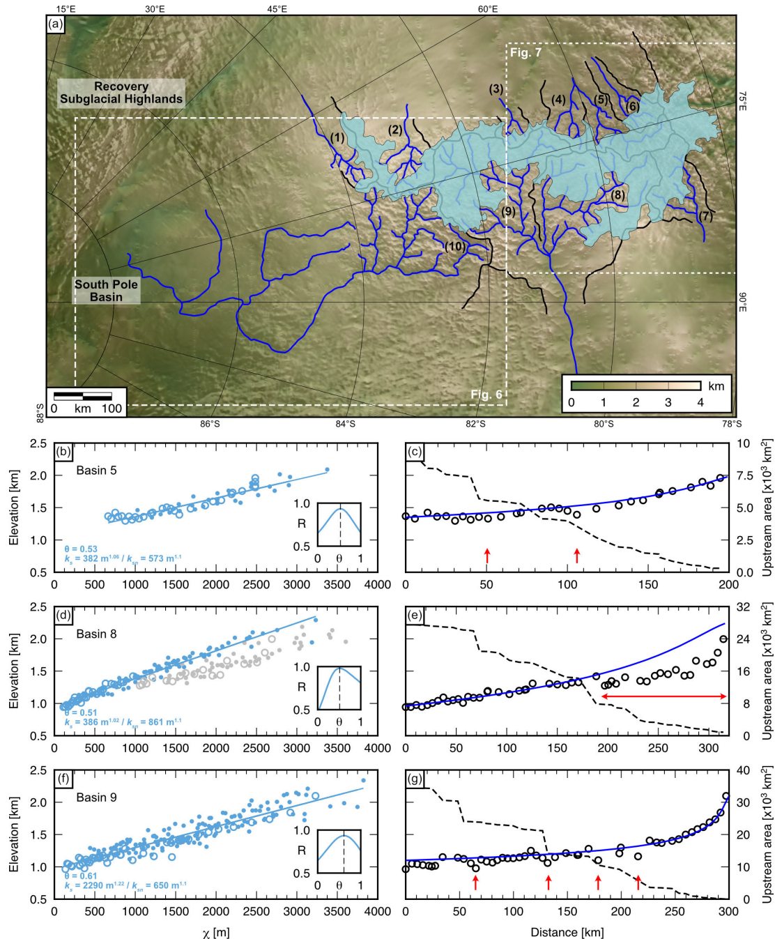
Figure 5. Relationship between Gamburtsev valley networks and mountain-scale glaciation at, or prior to, ca. 34 Ma. (a) Mapped GSM valley networks (blue lines) and drainage basin divides (black lines). Light blue shaded area marks the approximate mountain glacial limit at, or prior to, ca. 34 Ma, reconstructed using glacial geomorphological mapping (Rose et al., 2013). Bed elevations are derived from the rebounded Bedmap3 DEM (Paxman et al., 2022; Pritchard et al., 2025); shading is from the RADARSAT RAMP AMM-1 SAR image mosaic version 2 (Jezek et al., 2013). (b, d, f) \chi -elevation plots for basins 5, 8, and 9, respectively. Open circles = trunk valleys; closed circles = tributaries. Best-fitting \theta values are identified from the correlation coefficient ( R ; insets) of the linear regression (straight line). Recovered k_s and k_{sn} ( \theta_{\text{ref}} = 0.55 ) are labelled. (c, e, g) Corresponding theoretical fluvial longitudinal profiles calculated using Eq. (11) with the recovered \theta and k_s (blue line), superimposed on the observed trunk profiles (circles). Dashed line denotes upstream drainage area. In panel (d), grey circles mark points that deviate from the linear part of the plot, corresponding to the section of the profile marked by the horizontal red arrow in panel (e). Vertical red arrows mark deviations below the theoretical fluvial profile (overdeepenings), which often correspond with step-increases in upstream drainage area (i.e., tributary junctions).
