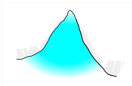
(ii) Permafrost change
