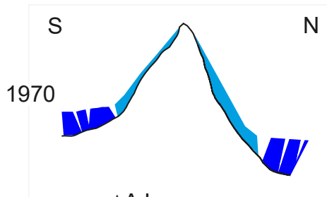
(i) Surface ice changes & geomorphic changes
