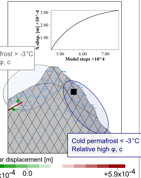
(b) UDEC model with shear parameters \phi(T) & c(T)
