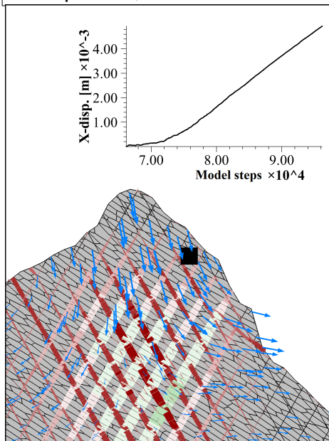
(c) \phi = 30^\circ , c = 0.1 MPa
