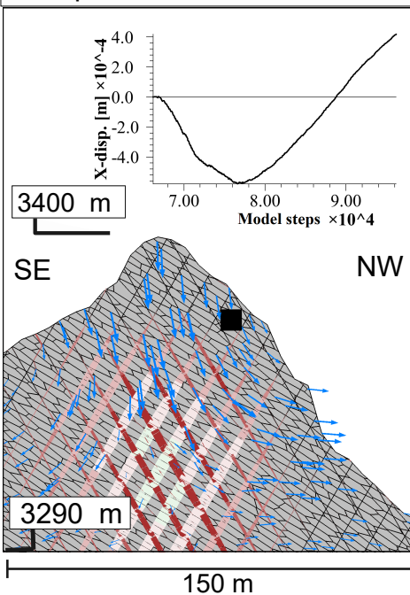
(b) \phi = 30^\circ , c = 0.2 MPa
