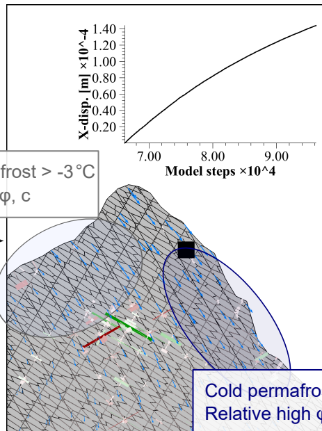
(b) UDEC model with shear parameters \phi(T) & c(T)
