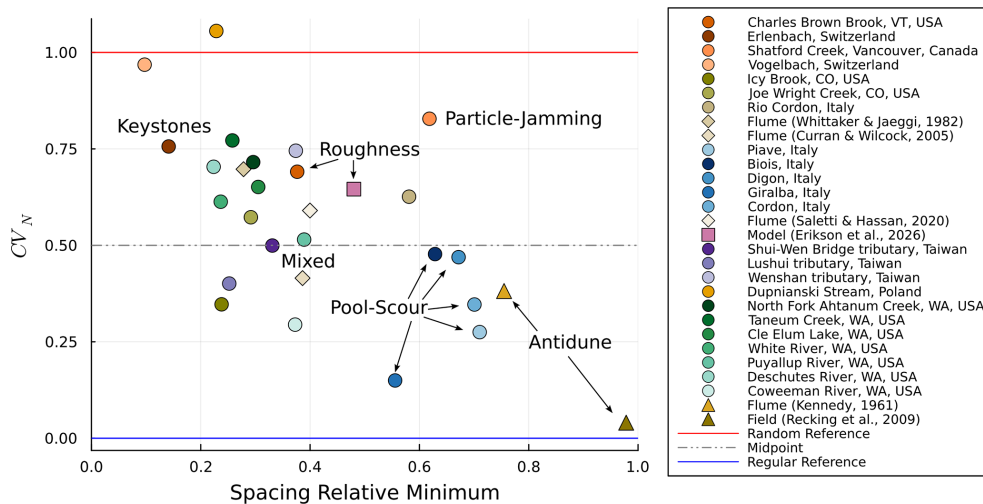
Figure 3. Mean positions in Fig. 2 averaged by source shown relative to the space between reference lines. The Range Normalized Coefficient of Variation ( CV_N ) is the y-axis of Fig. 2 now normalized by the y-axis space between the red and blue lines in Fig. 2 to show where within the envelope points occur (Eq. 1). The upper and lower lines are the same random and regular reference lines in Fig. 2, now in normalized space, and the dashed and dotted gray line indicates the middle point between them.
