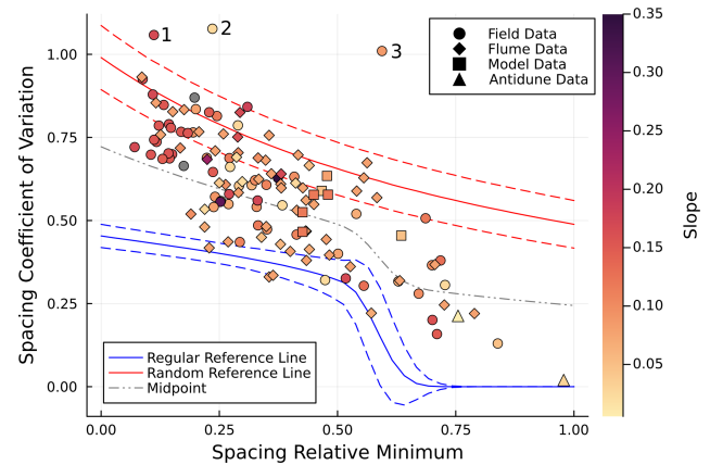
Figure 2. Comparison of data compiled from field, flume, and model step-pool spacing using a diagnostic plot ( n = 131 ). All points are colored by the slope of the reach in which observations were recorded, with gray points lacking slope information. Solid lines indicate mean values from a Monte Carlo simulation serving as a reference for regular (blue) and random (red) sequences and also correspond to values of CV_N = 0 and CV_N = 1 , respectively (see Fig. 3). Dashed lines represent one standard deviation in each direction from the estimated mean. The gray dotted and dashed line is the midpoint between the two reference lines. The three points above the random reference line are sequentially labeled. Point 1 is from large wood steps in the Vogelbach (Switzerland), Point 2 is from Charles Brown Brook (USA) after a flood, and Point 3 is from a reach of Shatford Creek (Canada) also featuring large wood.
