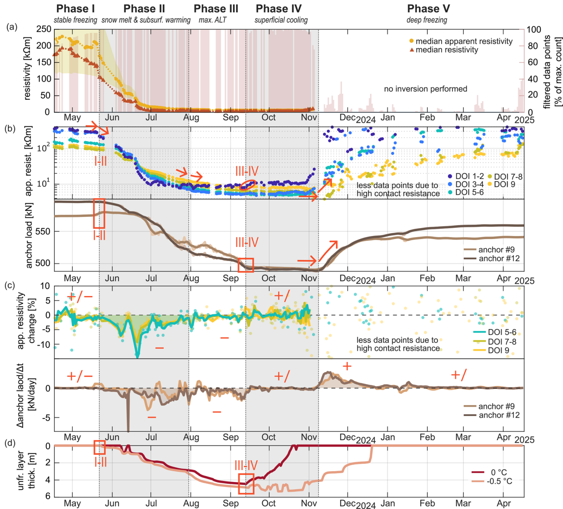
Figure 4. (a) Median apparent resistivity with interquartile range (yellow shading). Salmon bars indicate the percentage of available data points ( n = 135 ) after filtering. (b) Median apparent resistivity for specific depths of investigation (DOI) and raw as well as one-week-smoothed anchor load variations. (c) Relative changes in median apparent resistivity from deep-reaching ERT signals (DOI 5–9), smoothed over one week, and the rate of change (first derivative) of anchor loads. (d) Evolution of the unfrozen layer thickness based on the 0 and -0.5^{\circ}\text{C} isotherms. Red rectangles and arrows indicate the shifts in the parameter's pattern between the seasonal phases.
