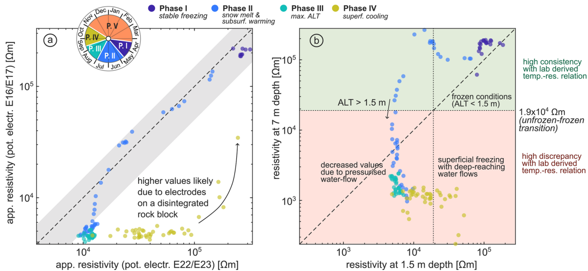
Figure 6. (a) Influence of small-scale rock heterogeneity on apparent resistivity, illustrated by a log–log plot comparing quadrupole measurements using potential electrodes E22/E23 (positioned on a disintegrated rock block) with E16/E17 (located at the profile centre). The grey band indicates a \pm 50\% deviation from the 1 : 1 line. (b) Median resistivity values at depths representative of permafrost conditions (7 m) and seasonally unfrozen conditions (1.5 m). The timing at which the active layer depth exceeds 1.5 m is marked. The transition between the unfrozen and frozen conditions at \sim 19 \text{ k}\Omega\text{m} is derived from laboratory experiments, see Offer et al. (2025) and Fig. 5.
