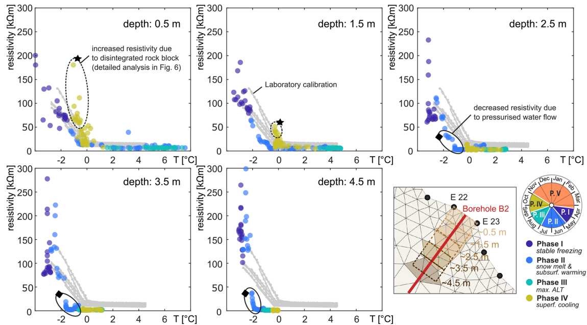
Figure 5. Seasonal and depth-dependent temperature–resistivity relationship combining (i) laboratory-derived resistivity experiments on core samples from the study site (grey lines, see Offer et al., 2025 for details) and (ii) field observations. Field data are plotted as median resistivity values for defined zones of interest along the borehole B2. Data points that deviate markedly from the laboratory relations are highlighted: deviations near the surface are attributed to likely high electrode contact resistance caused by surface drying or cooling of a disintegrated rock block, whereas high discrepancies at greater depths (2.5–4.5 m) coincide with periods of pressurised water flow.
