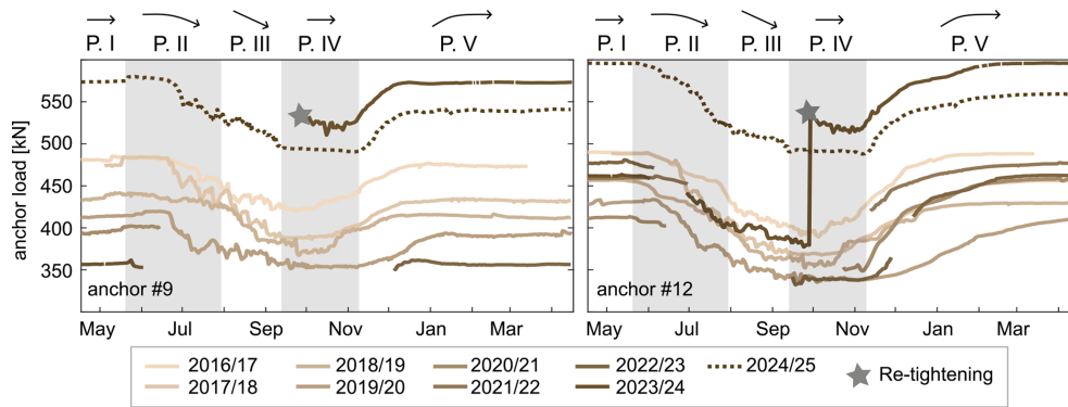
Figure A3. Seasonal patterns in anchor loads since the start of monitoring in 2016. High loads during phase I (stable freezing) are followed by a progressive decrease through phases II (snow melt and subsurface warming) and III (maximum active layer thickness), with minimum values typically observed in late summer in phase IV (superficial cooling). Loads increase again during phase V (deep freezing). The period of automated ERT monitoring between April 2024 and April 2025 is highlighted by a dashed line. Anchor re-tightening events are indicated.
