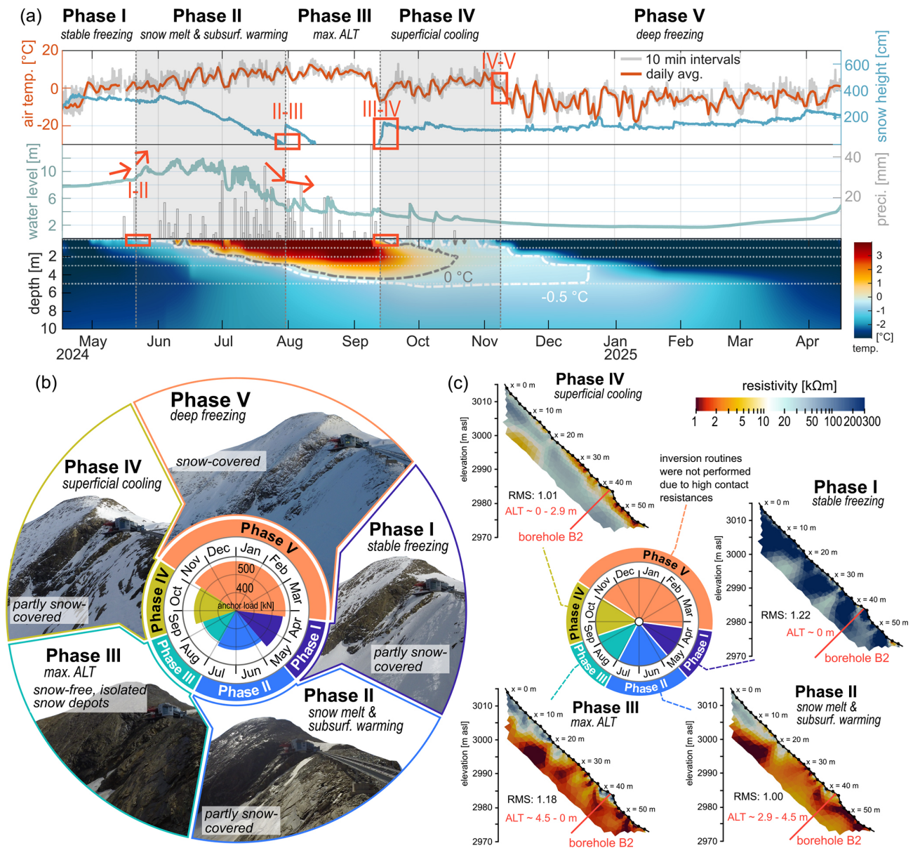
Figure 3. (a) Seasonal phases delineated by temporal shifts in environmental forcing (red rectangles and arrows), shown through air temperature, snow height (smoothed over 2 h), water levels from piezometric measurements, daily sum of precipitation on days with mean air temperatures > 2^{\circ}\text{C} (rainfall events), and spline-interpolated rock temperature with indicated thermistor depths. (b) Mean anchor loads (centre) and webcam images of the rockwall from 2 May, 11 July, 8 August, 29 October, and 11 December 2024. (c) Representative ERT models for phases I–IV with indicated active layer thickness (ALT) range; inversions were not performed for phase V due to the limited number of measuring points. The colour scale of the ERT models is based on laboratory calibrations from Offer et al. (2025).
