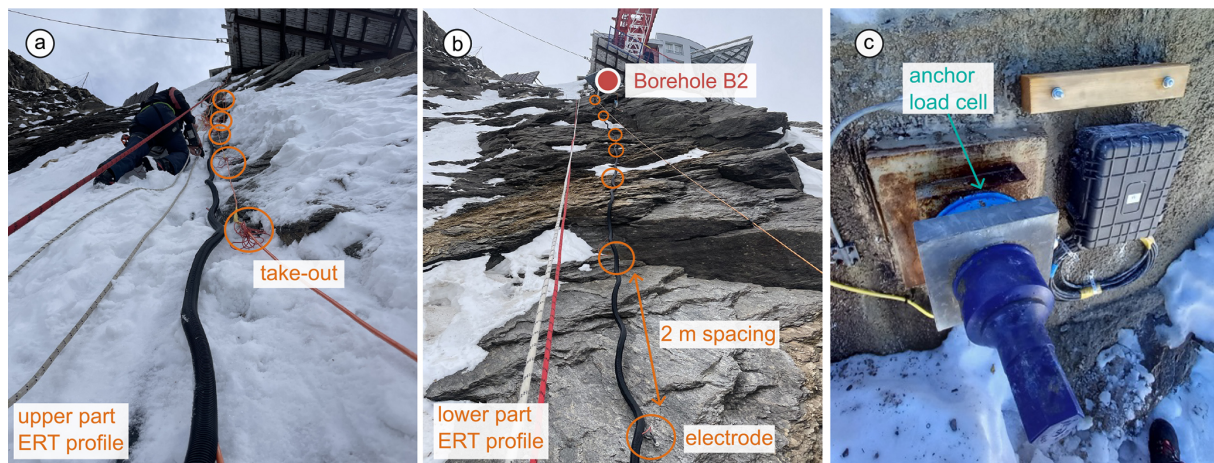
Figure A1. (a, b) Installation of the automated ERT monitoring with 2 m electrode spacing at the steep rockwall. The rock mass is characterised by pronounced discontinuities, including slope-parallel schistosity and several joint sets, which are particularly developed in the lower section of the profile. Borehole B2 is positioned along the ERT transect and was drilled through a disintegrated rock block. (c) Load-cell installation at the head of a 25 m long corrosion-protected anchor (18 m free length, 7 m friction-locked grouted), which primarily captures the relative strain variations between the activated rock mass and the free anchor length.
