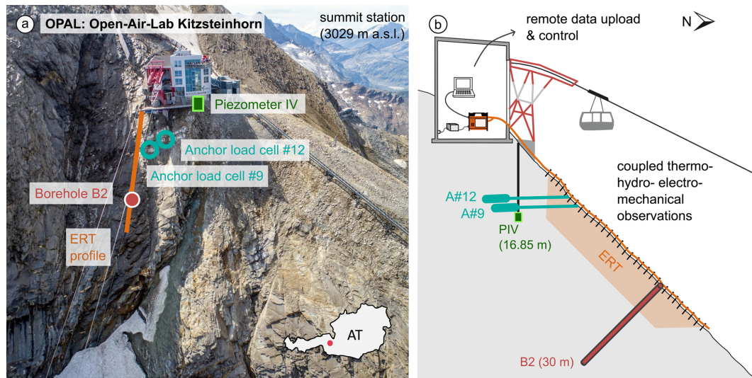
Figure 1. (a) Overview of the position of the instruments installed on the north flank of the Kitzsteinhorn: automated ERT setup at surface along the orange line, borehole temperature along the red profile, anchor load cells in turquoise, and piezometric measurements along a vertical borehole in green. (b) Schematic illustration of the vertical cross-section through the investigated rockwall from south to north, indicating the depths and inclinations of the monitoring systems.
