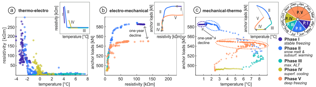
Figure A5. Electro-thermo-mechanical interaction of the rockwall with schematic representations for phases I–V: (a) Temperature–resistivity relation along borehole B2 down to 5 m depth, (b) resistivity–load relation based on the median apparent resistivity (from DOI 9, corresponding to a maximum electrode spacing of 18 m) and the mean load of both anchors, (c) temperature–load relation, represented by the mean anchor load and the temperature range (minimum to maximum) measured along the perpendicular anchor length (0–13 m). Dashed-line circles indicate periods when temperatures were entirely below 0 °C, making cryosuction unlikely. The one-year decline in anchor load is marked accordingly.
