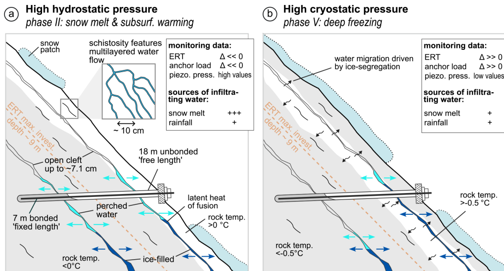
Figure 7. Schematic illustration of seasonal phases associated with high (a) hydrostatic and (b) cryostatic pressures that might predispose permafrost rockwalls to instability: (a) During snowmelt and subsurface warming (phase II), high hydrostatic pressure can develop above sealed fractures, leading to mechanically widening of fractures. (b) During deep freezing in winter (phase V), ice formation within discontinuities promotes ice segregation and associated cryostatic pressure build-up, resulting in stress redistribution within the rock mass.
