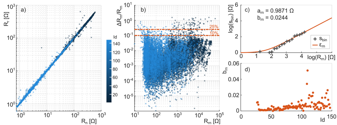
Figure 2. (a) Crossplot of normal and reciprocal resistance measurements of 18 018 data point pairs, showing a strong alignment along the 1 : 1 gradient with only a few outliers. (b) Relative reciprocal error ( \Delta R_{rn}/R_{rn} ), indicating that only isolated data points exceed the 10 % or 25 % thresholds, confirming the high quality of the raw data set. Measurements conducted during the winter and early spring months (Id = 0–60) exhibited higher relative reciprocal errors compared to summer observations (Id > 60), likely caused by increased contact resistance. (c) Determination of error model parameters a_m and b_m based on bin analysis of the standard deviation of the misfit between normal and reciprocal resistances ( \Delta R_{rn} ) and the mean resistance ( R_m ). (d) Temporal variation of the model parameter b_m across the time series, analysed separately for each ERT observation.
