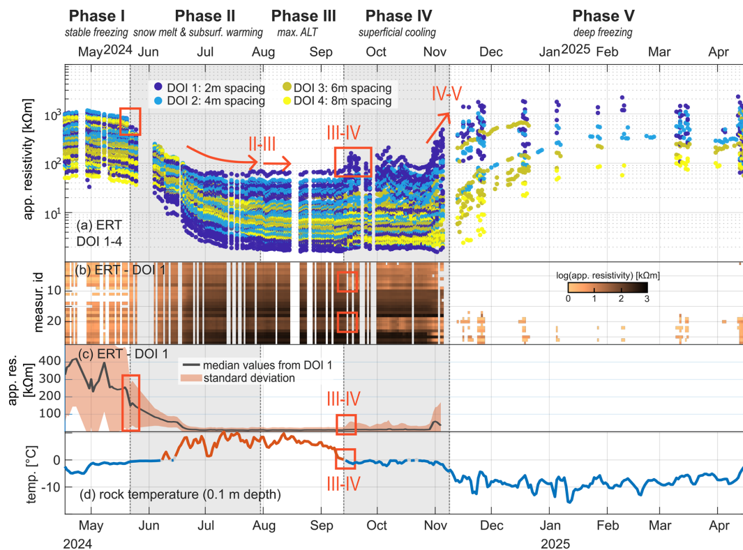
Figure A4. Apparent electrical resistivity and near-surface rock temperature: (a) Apparent resistivity in the upper subsurface layer measured with electrode spacing between 2 to 8 m (DOI 1–4). (b, c) Apparent resistivity near the rock surface with 2 m electrode spacing. (d) Rock temperature at 0.1 m depth in borehole B2, showing positive temperatures between early June and mid-September 2024. Red rectangles and arrows highlight shifts in parameter patterns corresponding to different seasonal phases.
