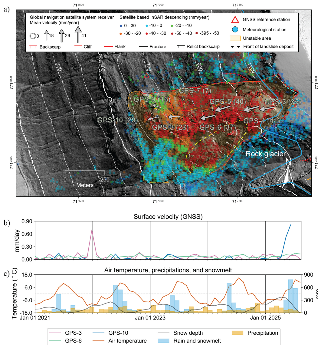
Figure 3. Overview of the Gámanjunki landslide. (a) Map illustrating key morphological features and instrument locations. Gray arrows denote mean GNSS-derived surface velocities ( \text{mm yr}^{-1} ) calculated for the period from 1 January 2021 to 12 August 2025, with arrow size scaled to velocity magnitude and annotated values in parentheses. The blue solid line indicates the elevation above which permafrost is highly probable (Etzel Müller et al., 2022). The yellow dashed outline delineates the active rock glacier extent. Elevation contours are shown in white at 100 m intervals. Hillshade based on Høydedata (© Kartverket). Accompanying plots display (b) GNSS velocity and (c) meteorological time series over the past five years. The GNSS velocity is calculated by a linear regression over one day and smoothed by down-sampling to 30 d median intervals, while the rainfall, snowmelt, and total precipitation is down-sampled to 30 d cumulative intervals.
