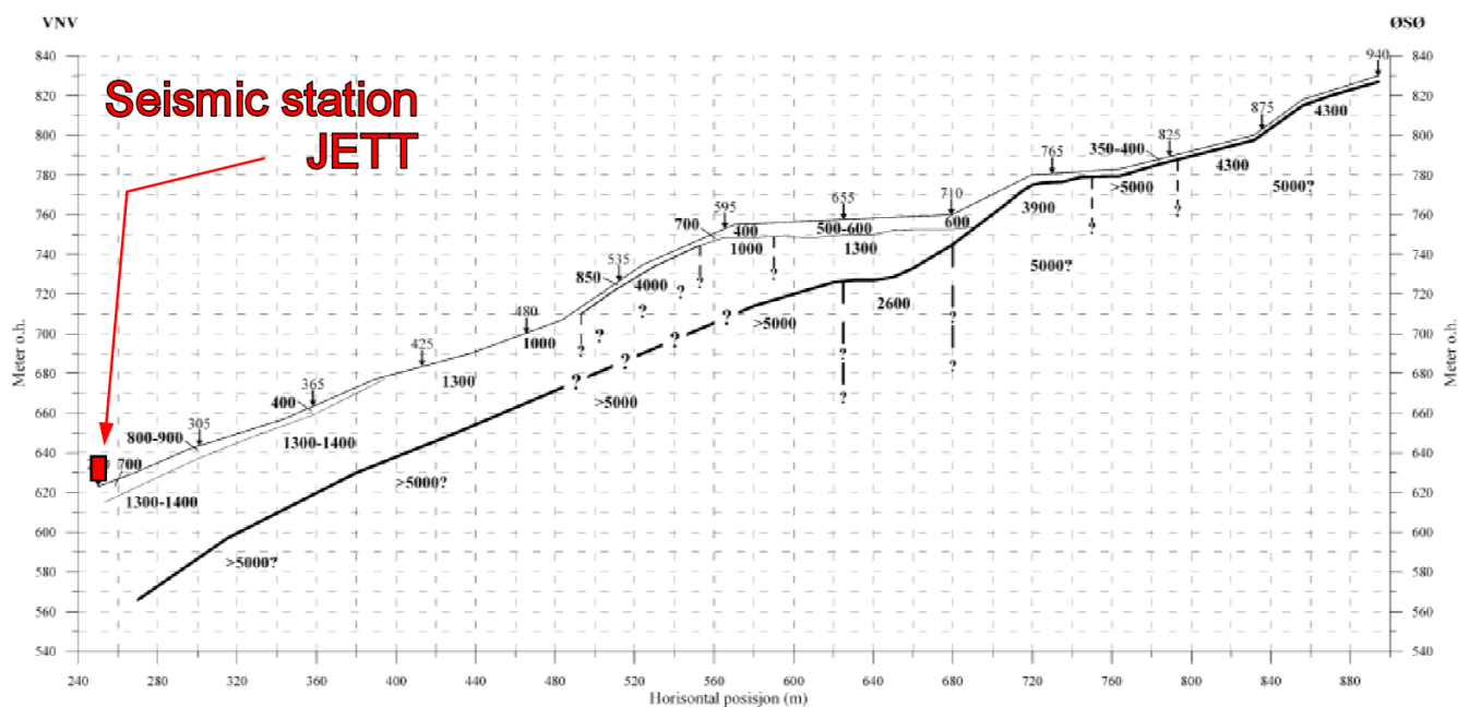
Figure A7. Seismic refraction profile in the upper part of the Jettan rockslide (Rønning et al., 2008). The location of the profile is shown in Fig. A6.
