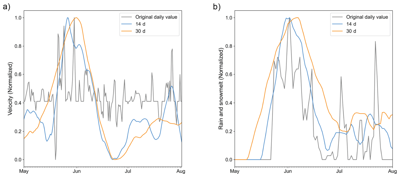
Figure A1. Verification of zero lag created by the window lengths by the rolling functions. (a) Normalized velocity from GPS-4 on Jettan with 1, 14, and 30 d velocity calculated by the centered rolling linear regression function (see Section Integration of Data). (b) Normalized rain and snowmelt summed over 1, 14, and 30 d by the centered running sum function.
