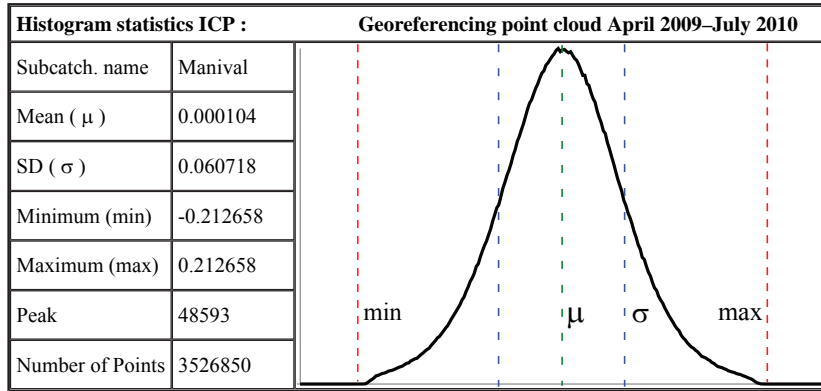
Figure 6. Distribution of the distance between two survey point clouds after the process of georeferencing using the ICP procedure. The distance approaches normal distribution with a zero mean, showing that errors generated by multiple scan registration and point cloud survey georeferencing are Gaussian, random, and independent. Data are given in metres.
