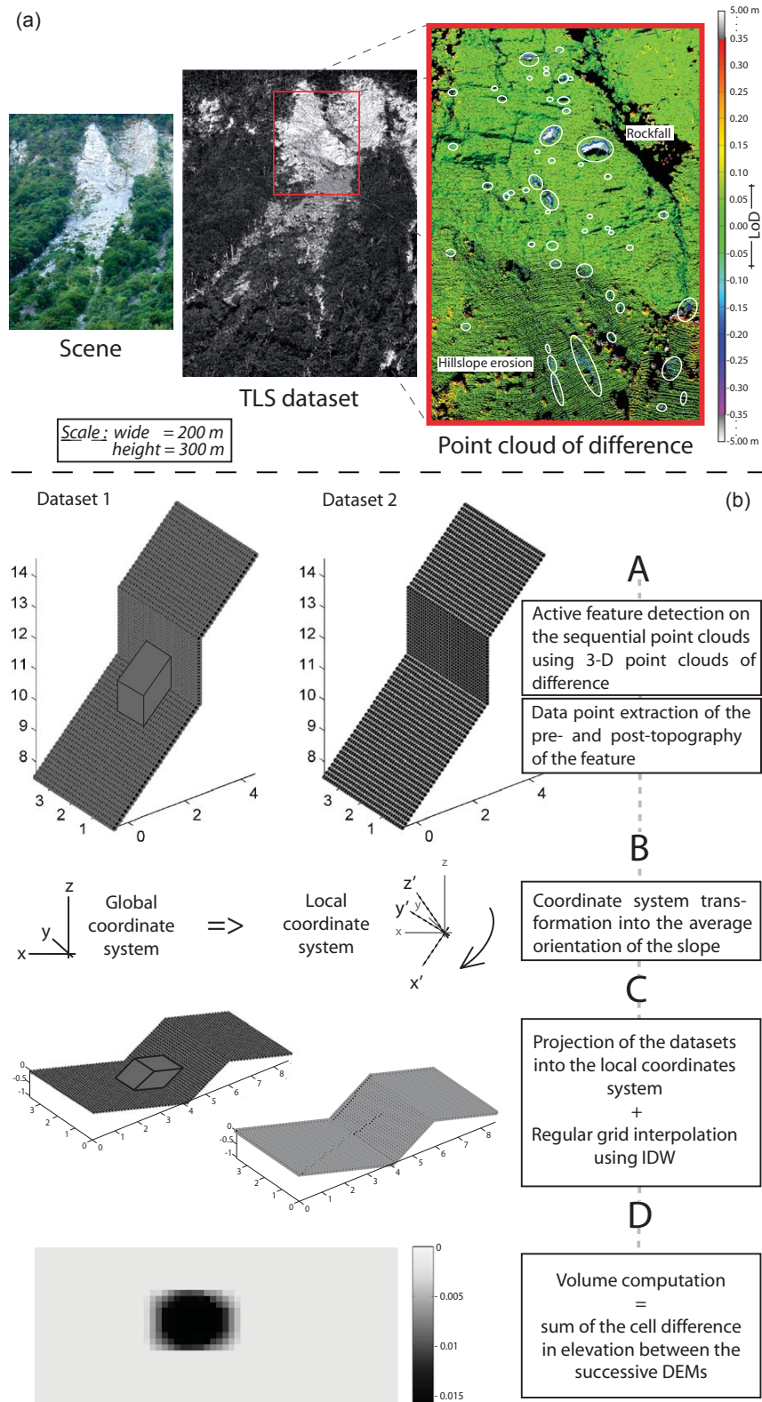
Figure 5. 3-D detection (a) and schematic illustration (b) of the extraction and volume computation method of an individual active feature provided by two successive point cloud datasets.
