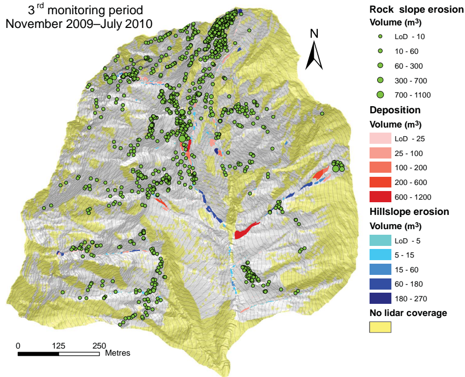
Figure 9. Geomorphic activity revealed by comparing the topographic differences of the two successive TLS surveys operated in November 2009 and July 2010. The sediment budgets for each subcatchment are detailed in Fig. 15.
