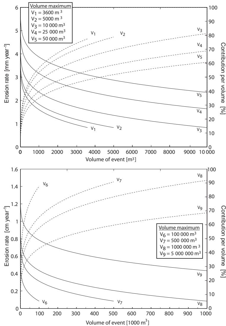
Figure 16. Continuous lines: erosion rate as function of size of events for a certain volume of production (potential maximum volume V_{1\dots 9} ), considering that rockfall volume distribution observed at Manival follows power law behaviour (Table 6). Dashed lines: contribution of each class of volumes to the erosion rate showing the significant effect of large slope failures. For a maximum eroded volume of 3600\text{ m}^3\text{ yr}^{-1} ( V_1 ), the 1000\text{ m}^3 rockfall event contributes 60 %, while events less than 100\text{ m}^3 induce less than 20 % of erosion, although they are of a much higher frequency; a 100\,000\text{ m}^3 rockslide would generate 70 % of total eroded material of 500\,000\text{ m}^3 ( V_7 ) over a century.
