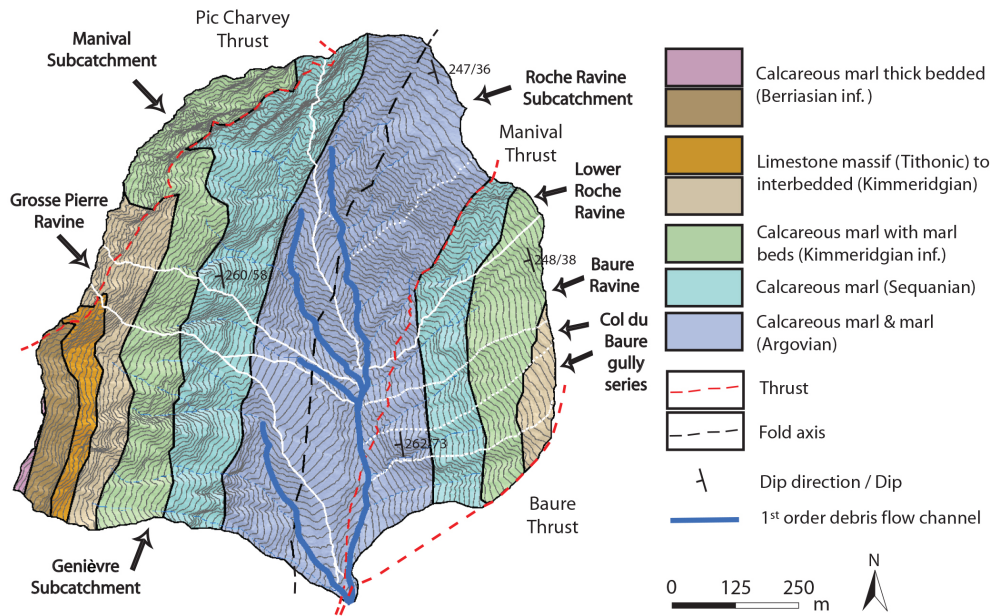
Figure 2. Geological map of the catchment headwater (production zone) after Gidon (1991) and location of first-order debris flow channels (thick blue line) and their respective watersheds (white lines). For the ease of analysis, the Roche Ravine and Col du Baure subcatchments in the east side were further subdivided according to their gully complex (dotted white lines).
