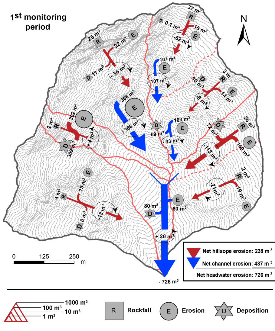
Figure 13. Overall headwater sediment budget observed during the first monitoring period revealing the sediment dynamics through the spring–summer season and the net balance of sediment recharge in the downstream torrent for several months preceding the August 2009 debris flow.
