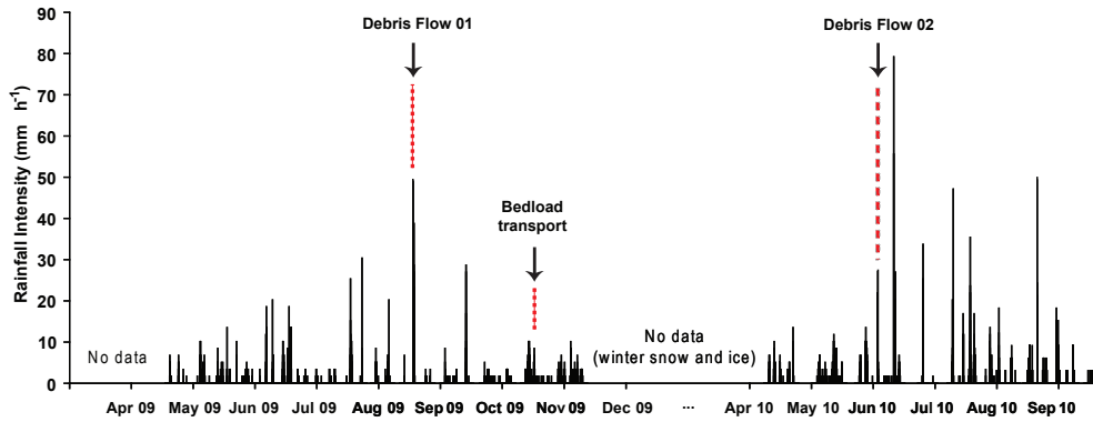
Figure 3. Maximum rainfall intensity over the monitoring period measured by a rain gauge located at the top of the torrent (see Fig. 4) and calculated for a 5 min time interval. The mean annual precipitation is about 1500 mm in the headwater of the Manival (modified from Loye, 2013).
