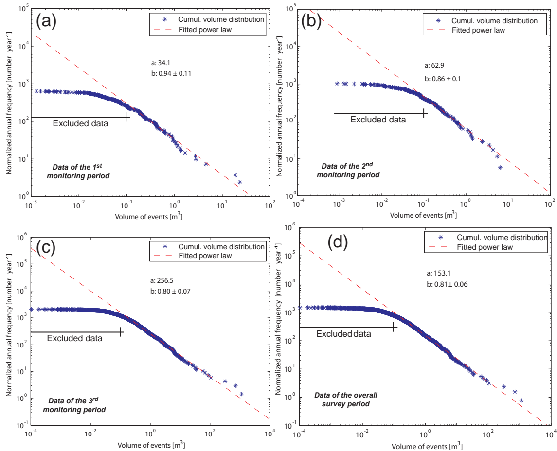
Figure 10. Cumulative volume distribution of the rockfall observed during the first (a), the second (b), and the third monitoring period (c) and over the entire study time of 16 months (d). For each dataset, the power law is fitted for volumes larger than 0.1 \text{ m}^3 . Below this threshold volume, the distribution exhibits a rollover that progressively reaches an almost constant frequency for the smallest detected volumes.
