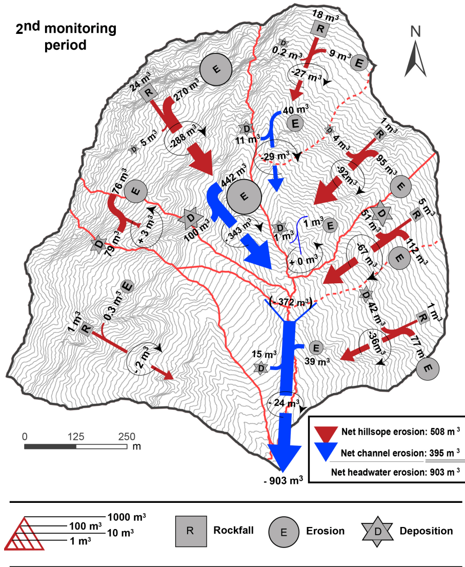
Figure 14. Overall headwater sediment budget observed during the second monitoring period revealing the sediment dynamics and the net balance of sediment recharge in the downstream torrent during the autumn.
