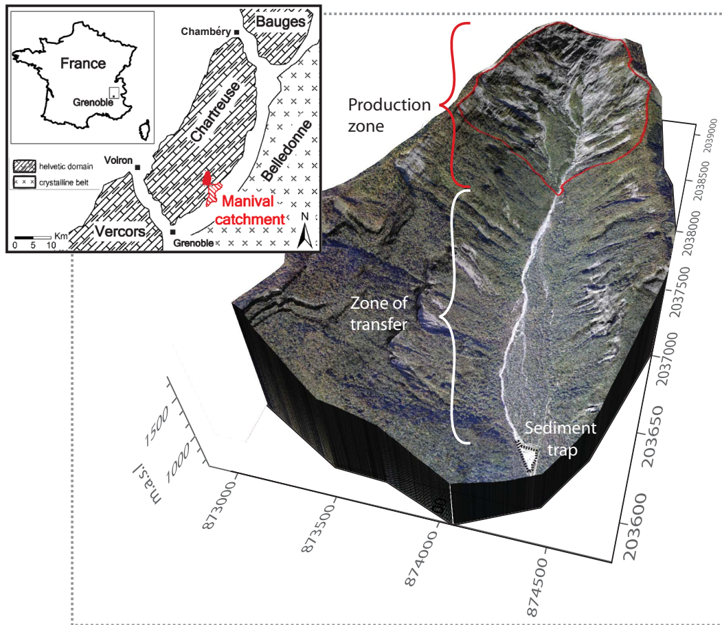
Figure 1. Inset: map of the study area; the Manival catchment is in solid red and the impressive debris fan is hatched. Main: aerial view of the Manival catchment, draped over a topographic model; sediment supply is concentrated in the headwater (production zone) as erosion activity from the middle and lower catchment is not connected to the torrent (zone of transfer) (image: Aerodata International Surveys; DEM: Irstea UR ETNA).
