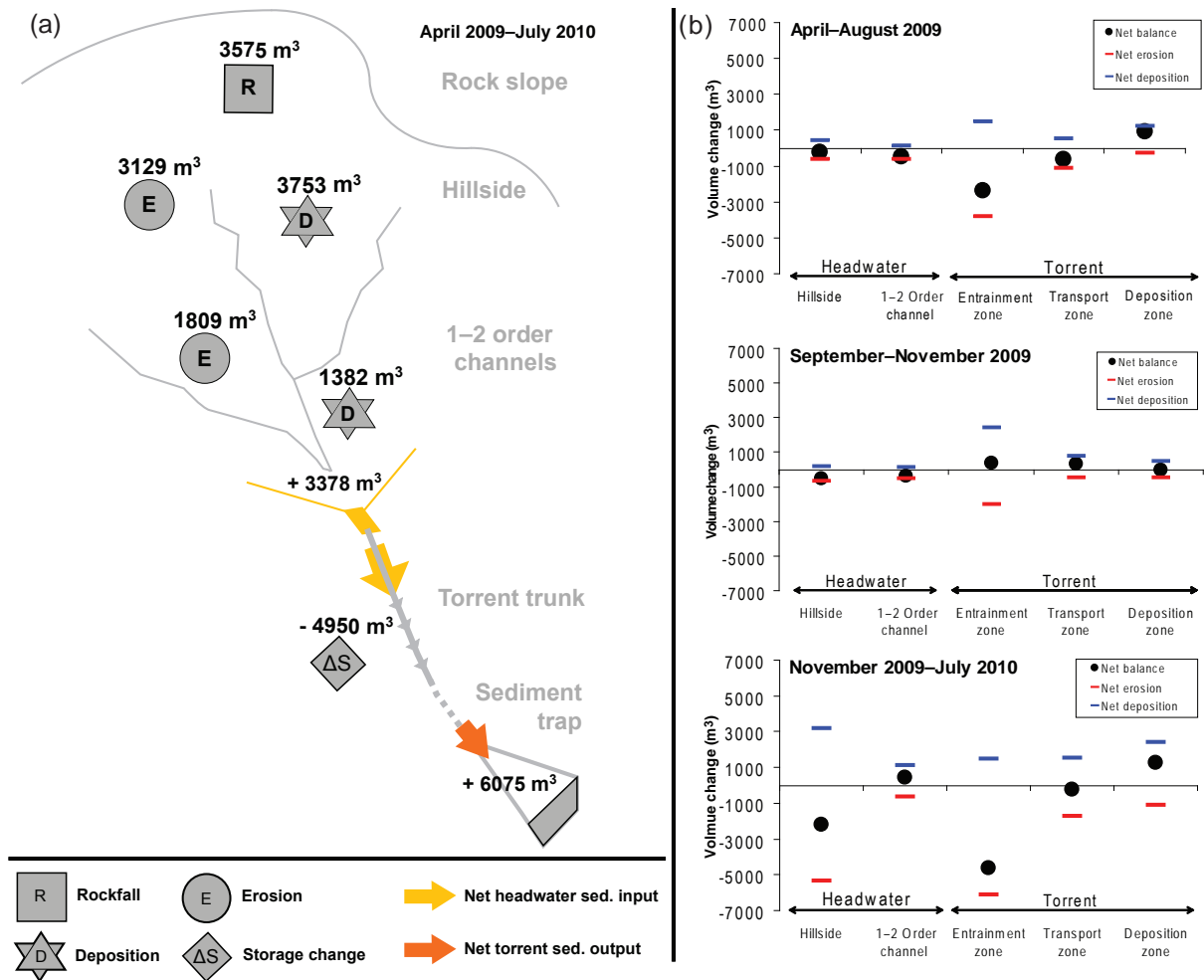
Figure 12. Overall sediment budget (a) and net sediment balance (b) for each monitoring period showing the overall transfer dynamics from debris source zone in the headwater to the apex of the fan through the torrent observed during the period of investigation.
