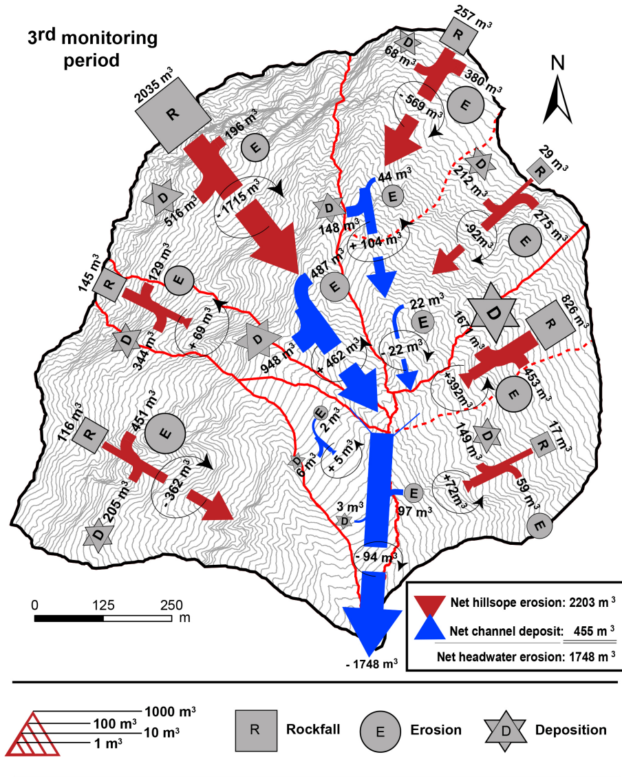
Figure 15. Overall headwater sediment budget observed during the third monitoring period revealing the sediment dynamics through the winter–spring and the net balance of sediment recharge in the downstream torrent for the period preceding the June 2010 debris flow.
