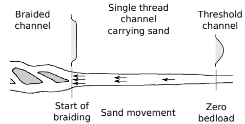
Figure 4. Transient channel in Stebbings' experiment (reproduced from Stebbings, 1963). Flow from right to left.
