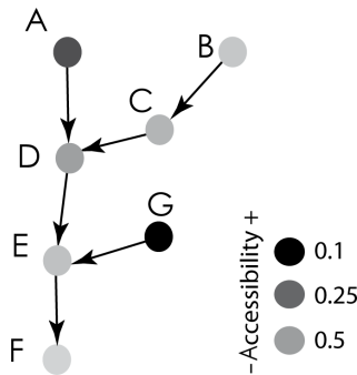
Figure 3. Assessment of the accessibility index (Shi) within the virtual sediment cascade.
