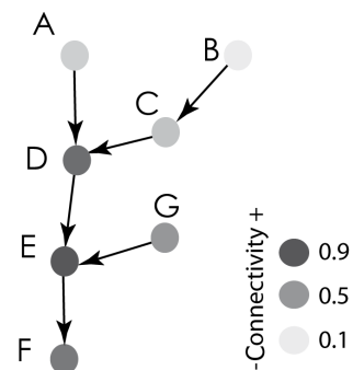
Figure 4. Assessment of the connectivity within the virtual sediment cascade using the NSC index.
