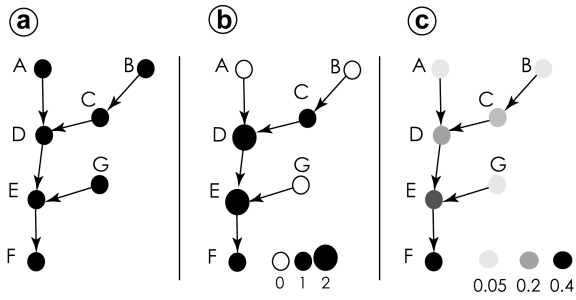
Figure 2. The virtual sediment cascade. (a) The structure of the cascade, represented by a graph; all nodes are supposed equals in terms of sediment availability (spatially uniform sediments availability; virtual units = 1). (b) The potential flow of sediments after one iteration during the simulation (see also Table 3, column “1”); (c) map potential flux index ( F_i ) values (see also Table 3, column “ F_i ”).
