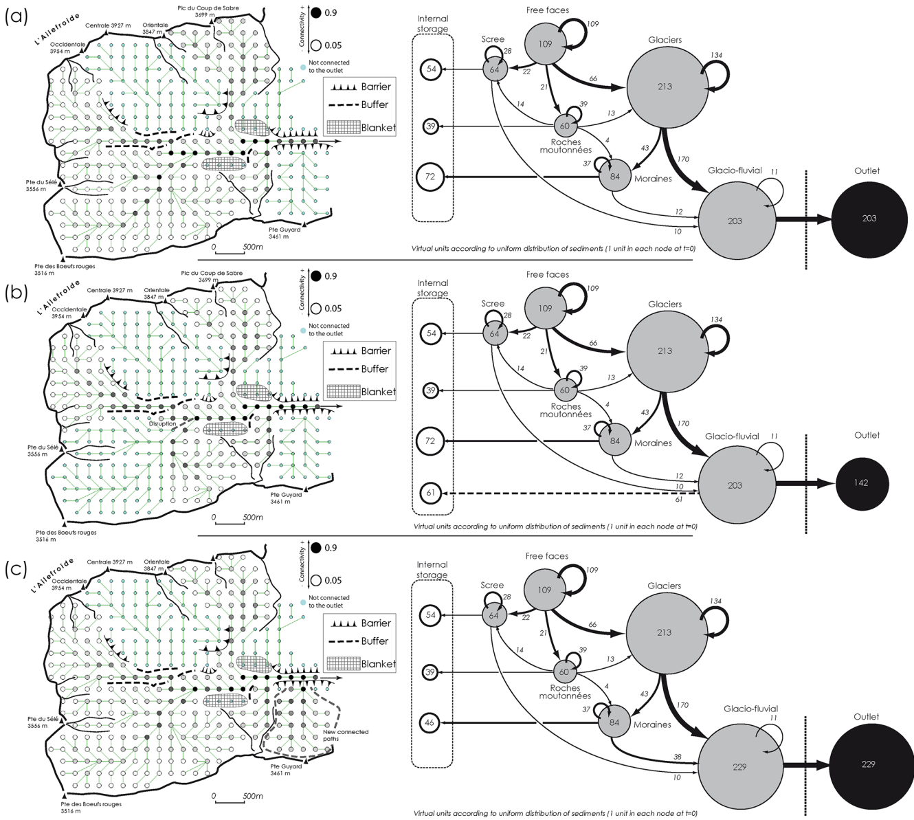
Figure 7. Assessment of connectivity. (a) Current structure of the cascade. (b) Connectivity map after the simulation of a disruption at Sélé toe. (c) Connectivity map after the simulation of a reconnection at Guyard outlet.
