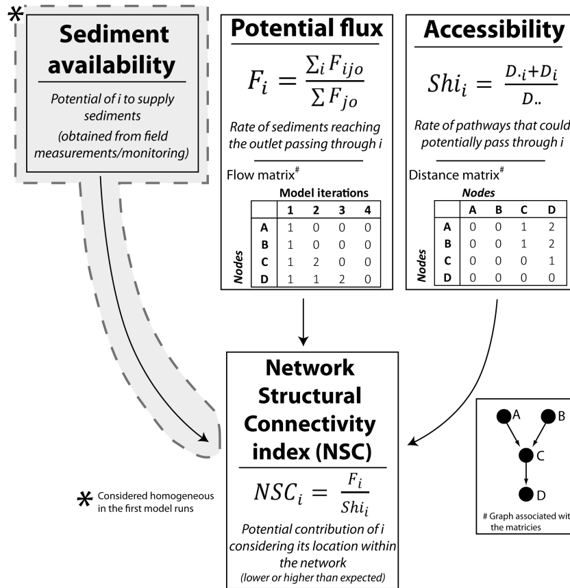
Figure 1. Overview of the main parameters used to build the network structural connectivity index (NSC) (equation details can be found in Sect. 3).
