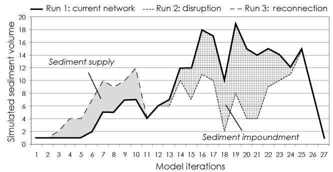
Figure 8. Sedimentographs associated with runs 1, 2 and 3 on Celse-Nière catchment. Run 1 shows the current effect of the spatial network structure on sediment waves, run 2 the potential impact of an edge disruption in a hotspot zone, and run 3 the potential impact of a reconnection. Runs 1, 2 and 3 correspond to the graphs in Fig. 7a, b and c, respectively.
