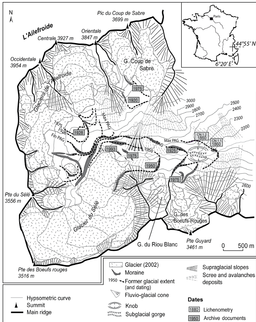
Figure 6. Geomorphological map of the study area: Celse-Nière catchment and sediment cascade.
