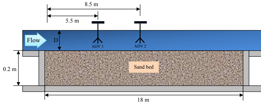
Figure 2. Schematic diagram of the experimentation flume showing the key dimensions and ADV locations.
