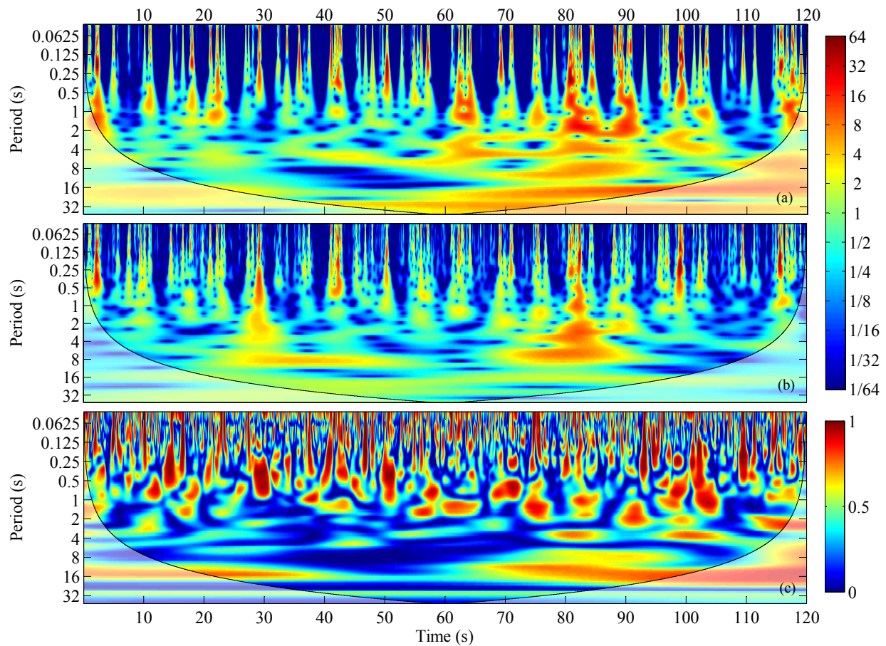
Figure 10. Wavelet power spectra (Morlet wavelet) for below the measured mean critical velocity experiment ( \bar{u} < \bar{u}_{cr, measured} ) for a 2 min period showing the (a) momentum flux ( u' , w' ), (b) sediment flux ( c' , w' ), and (c) coherence between the momentum and sediment fluxes.
