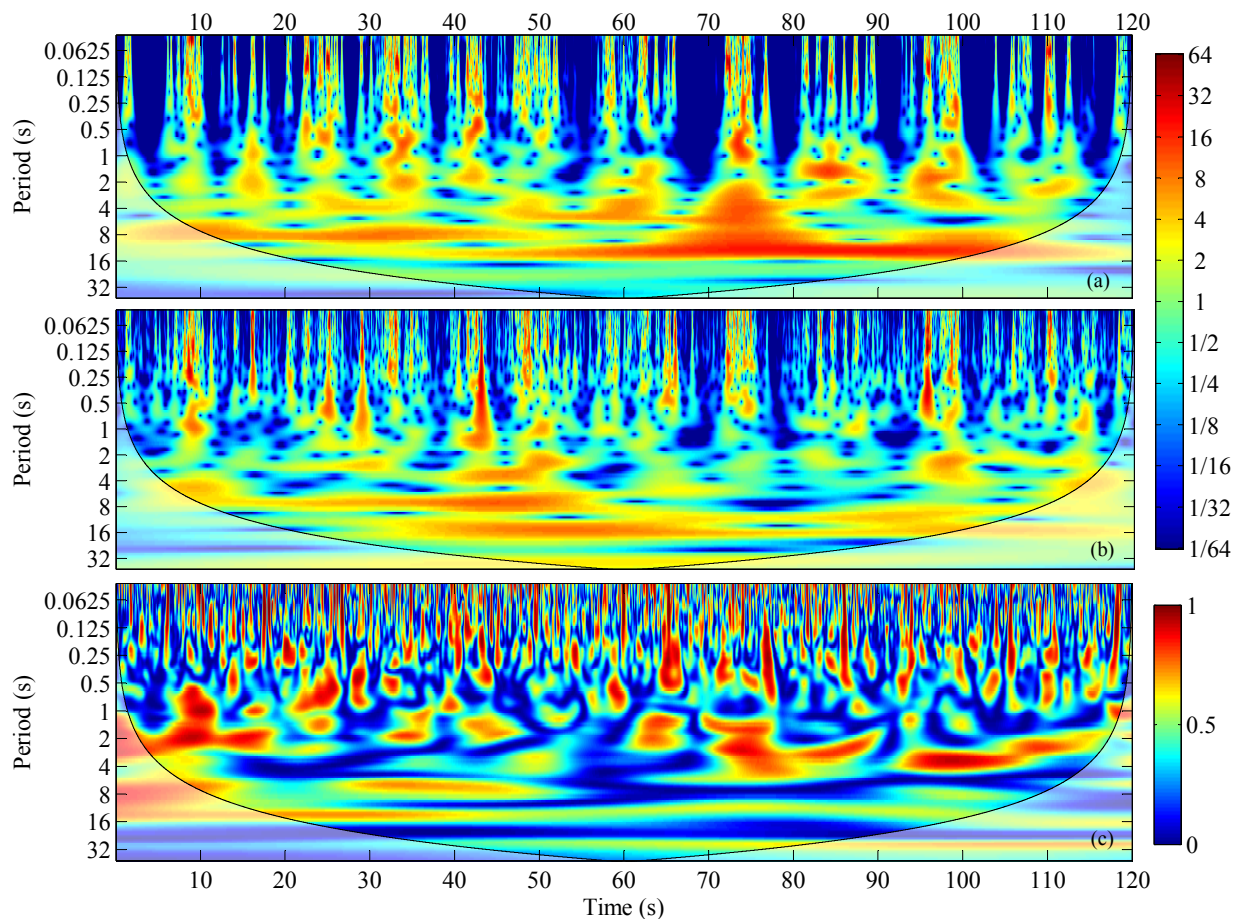
Figure 9. Wavelet power spectra (Morlet wavelet) for above the measured mean critical velocity experiment ( \bar{u} > \bar{u}_{cr, measured} ) for a 2 min period showing the (a) momentum flux ( u', w' ), (b) sediment flux ( c', w' ), and (c) coherence between the momentum and sediment fluxes.
