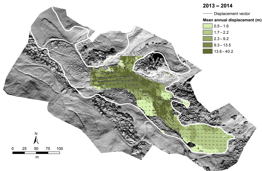
Figure 7. Surface displacements for 2013–2014 using the COSI-Corr algorithm. Displacement vectors are indicative of relative magnitude and direction of movement and do not reflect true ground displacements.
