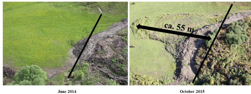
Figure 9. Aerial images illustrating the advance of the frontal lobe of the earthflow between June 2014 and October 2015.
