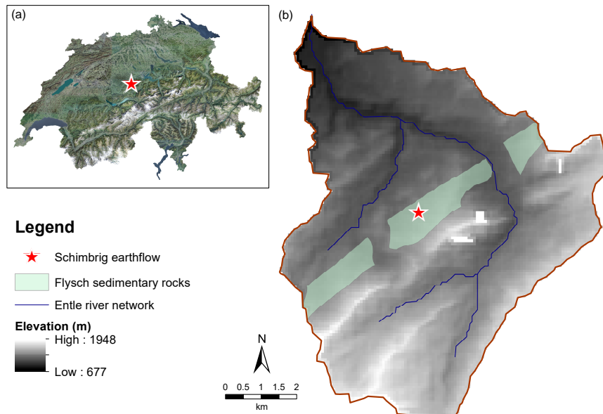
Figure 1. Location of the Schimbrig landslide in Switzerland (a) and in the Entle River watershed (b).
