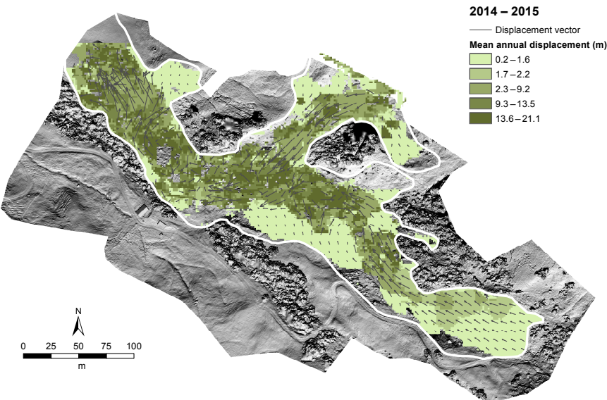
Figure 8. Surface displacements for 2014–2015 using the COSI-Corr algorithm. Displacement vectors are indicative of relative magnitude and direction of movement and do not reflect true ground displacements.
