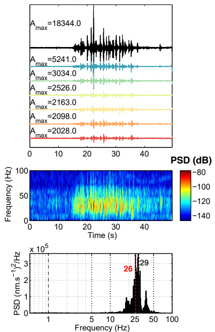
(e) Aaknes
