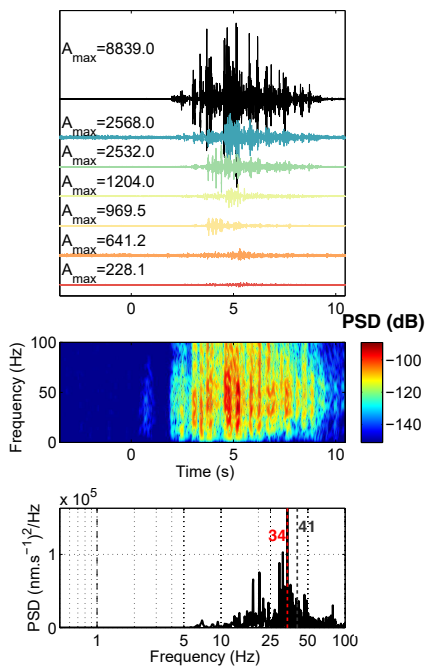
(e) Aaknes
