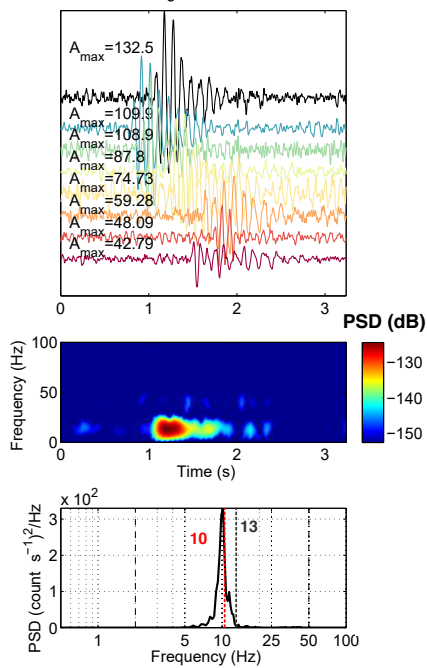
(e) Slumgullion
