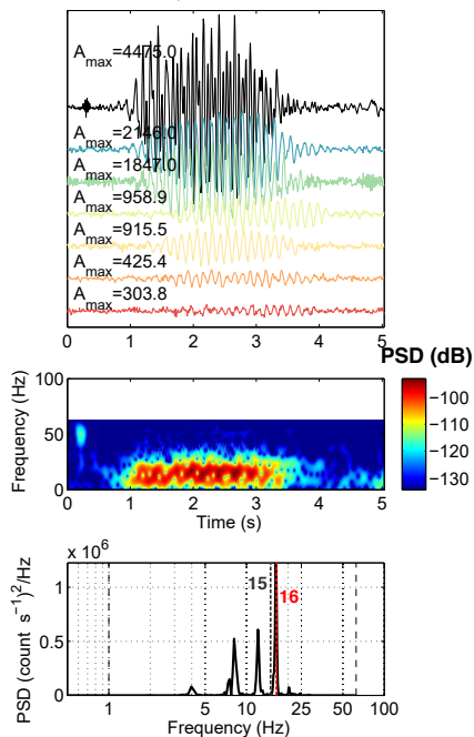
(e) Slumgullion
