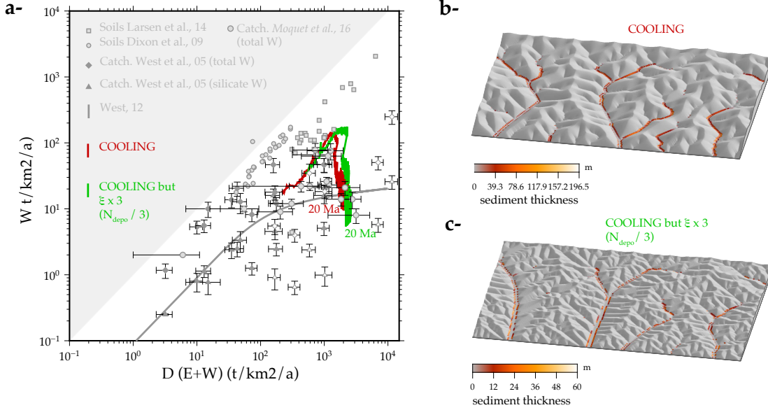
Fig. S4: Effect of increasing the transport length coefficient \xi by 3 ( N_{\text{depo}} / 3 ) in experiment COOLING. \alpha=0.001 . (a-) Increasing the transport length, there is less deposition. Consequently, the sediment thickness in valley borders is smaller and the weathering outflux associated with colluvium is lower. The second effect of increasing the transport length is to increase the lateral erosion. Indeed, lateral erosion is proportional to the sediment flux. The sediment flux is greater if there is less deposition, thus the lateral erosion increases. Consequently, rivers are more straight and the residence of sediment in the river is shorter. This second effect contributes also to lower the weathering outflux associated with the weathering of colluvium. Note that the relief in the experiment with \xi \times 3 appears less realistic than in the COOLING experiment. Yet, the colluvial deposits produce all the weathering outflux during the cold period. This comparison illustrates that the weathering outflux follows the same humped evolution passing by a maximum weathering outflux and then that colluvial deposits produce a significant weathering outflux, although the value of this flux is lower for smaller N_{\text{depo}} . (b-) Topography (relief \times 2 ) and sediment thickness at 20 Ma for the COOLING experiment. (b-) The same for \xi \times 3 ( N_{\text{depo}} / 3 ).
