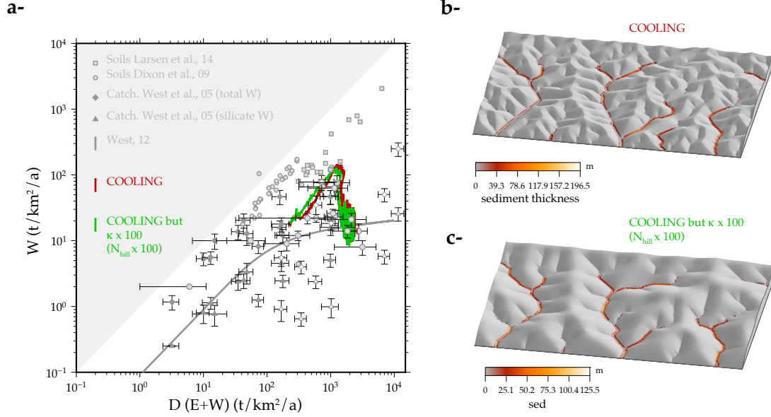
Fig. S3: Effect of increasing the diffusion coefficient \kappa by 100 ( N_{hill} \times 100 ) in experiment COOLING. \alpha=0.001 . (a-) Despite different values for the non-dimensional parameter N_{hill} , the weathering outfluxes follow similar evolutions. This comparison illustrates that the weathering outflux follows the same humped evolution passing by a maximum weathering outflux and then that colluvial deposits produce the same significant weathering outflux whatever N_{hill} is. (b-) Topography (relief \times 2 ) and sediment thickness at 20 Ma for the COOLING experiment. (b-) The same for N_{hill} \times 100 .
