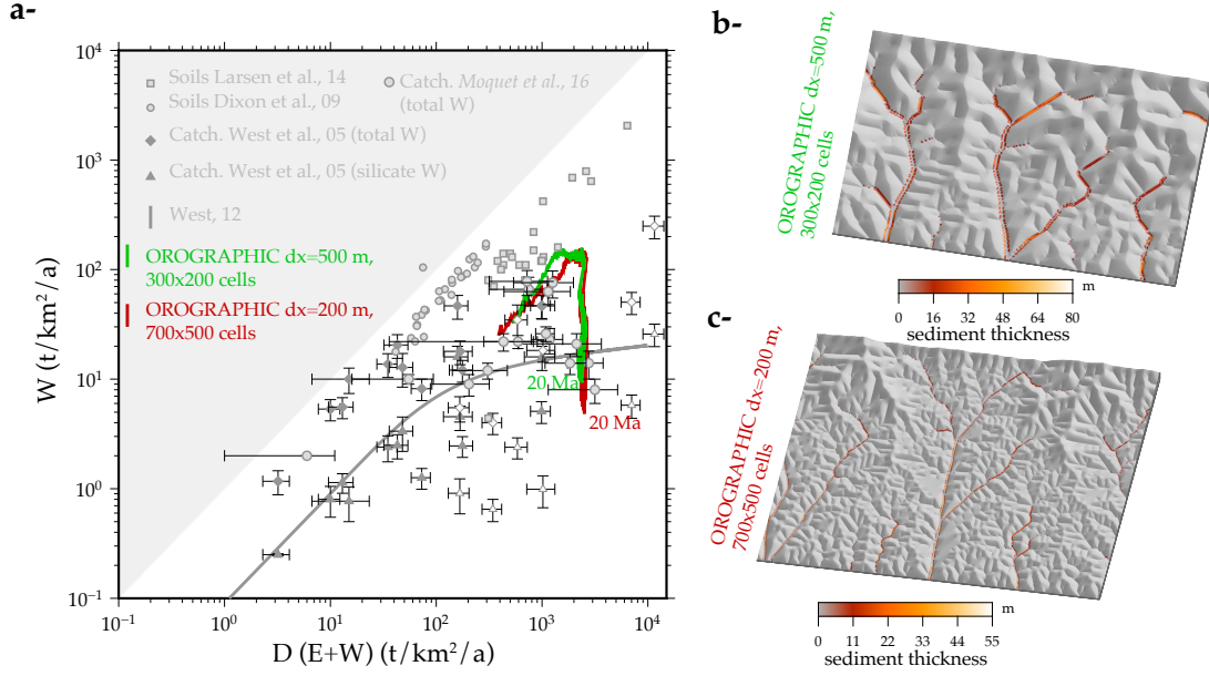
Fig. S5: Effect of increasing the model resolution for experiment OROGRAPHIC with a rainfall peak at 2000 m. The experiment OROGRAPHIC presented in the main manuscript has 300x200 cells of size 500 m. The other experiment has 700x500 cells of size 200 m. The lateral erosion parameter \alpha is 2.5 times smaller. (a-) The weathering rate follows a similar evolution in both cases, but the experiment with the smaller cells ends up with a smaller weathering rate associated with colluvium weathering, resulting from the smaller lateral erosion parameter decreasing the volume of colluvium. This comparison shows that decreasing the cell size does not change fundamentally the fact that the weathering outflux follows the same humped evolution passing by a maximum weathering outflux and then that colluvial deposits produce a significant weathering outflux during the cold period, even in a more penalizing experiment with smaller lateral erosion. (b-) Topography and sediment thickness at 20 Ma in the OROGRAPHIC simulation using dx=500 m. (c-) The same for the OROGRAPHIC simulation using dx=200 m.
