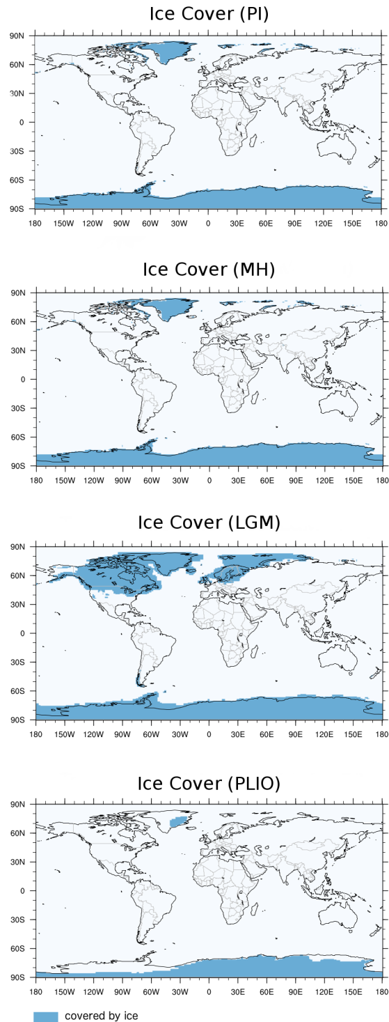
Figure S1: ice cover reconstructions used for PI, MH, LGM and PLIO simulations.
