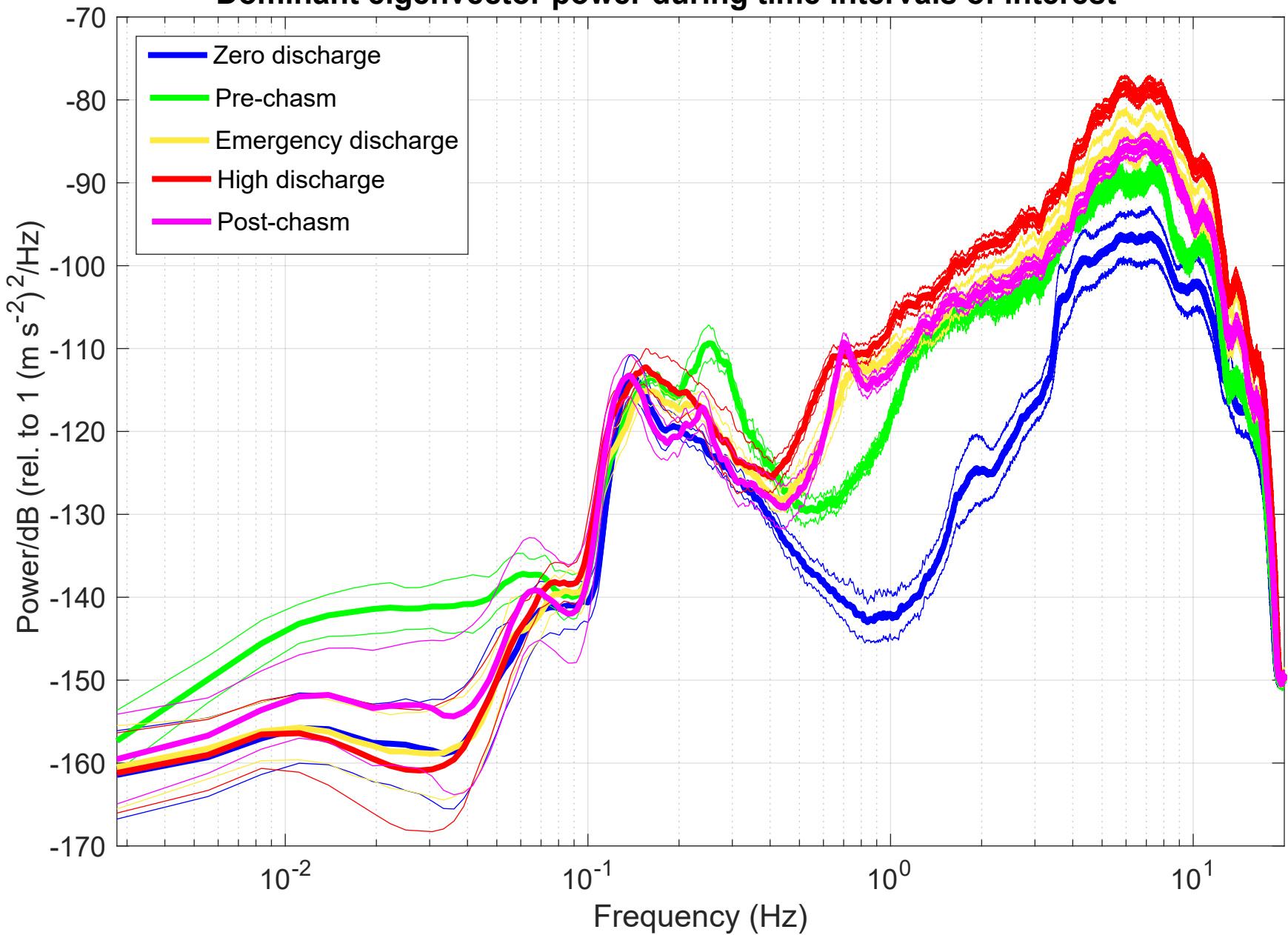
Dominant eigenvector power during time intervals of interest
