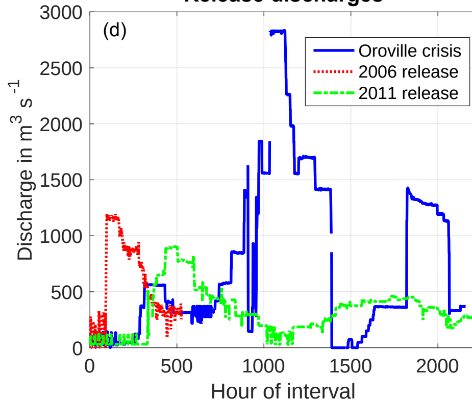
Release discharges
