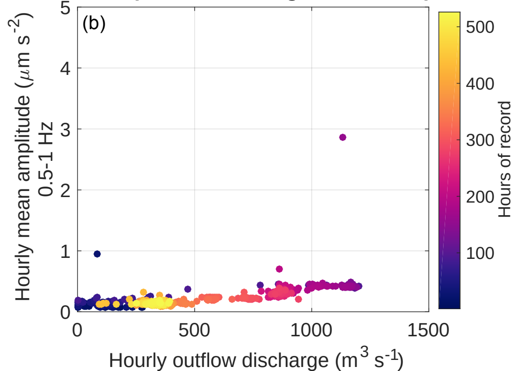
2006 amplitude-discharge relationship
