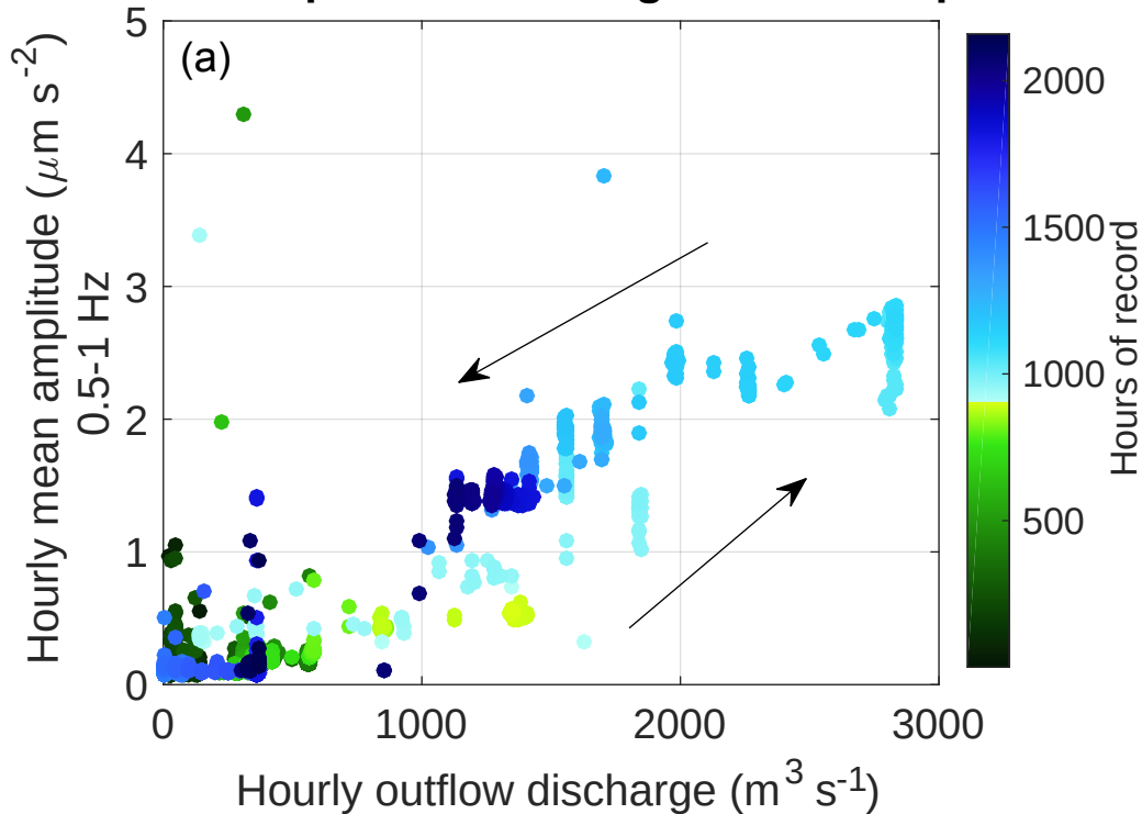
2017 amplitude-discharge relationship
