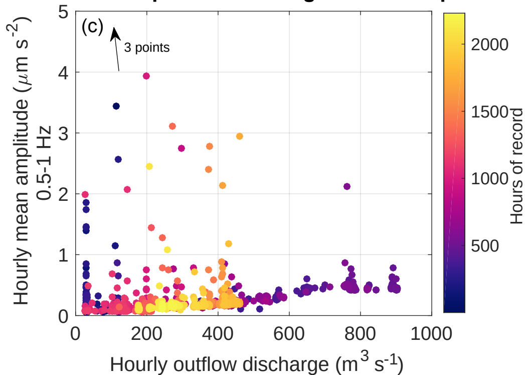
2011 amplitude-discharge relationship
