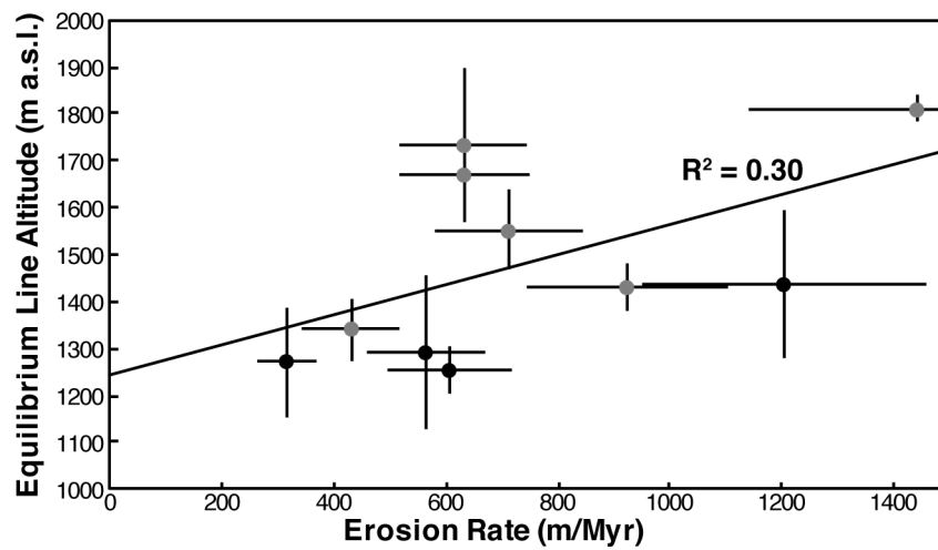
Figure S2. Comparison of basin-averaged erosion rates and equilibrium line altitudes. Black and grey data are from the west and east sides of the range, respectively.
