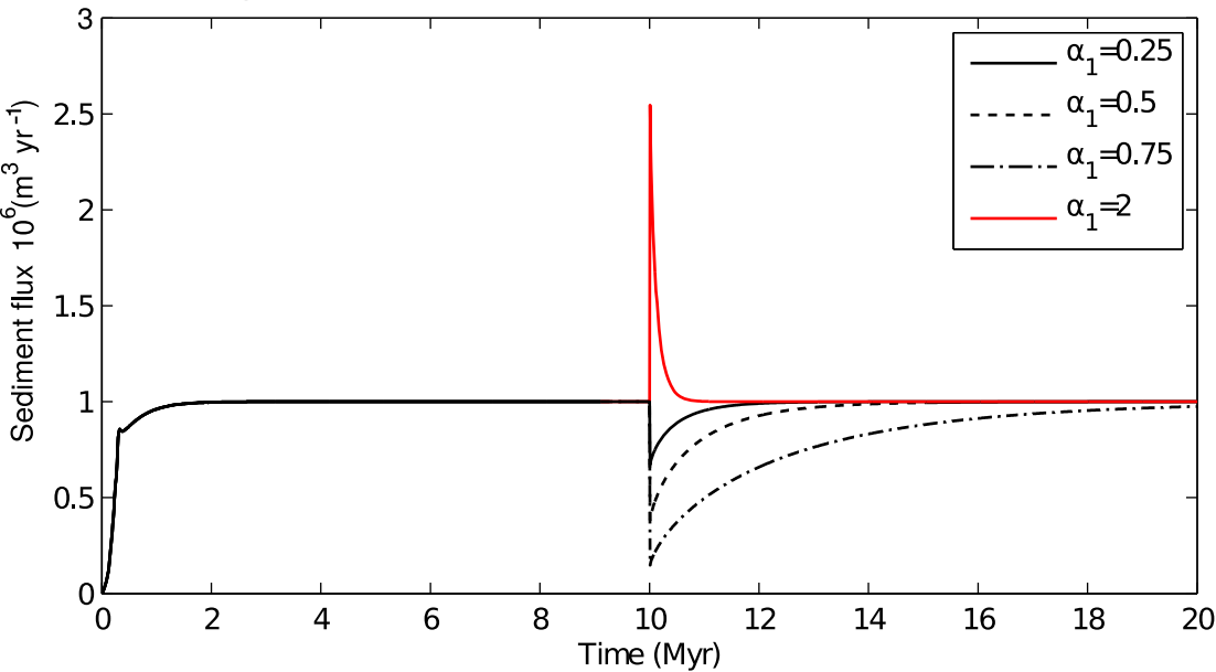
(b) Stream power model
