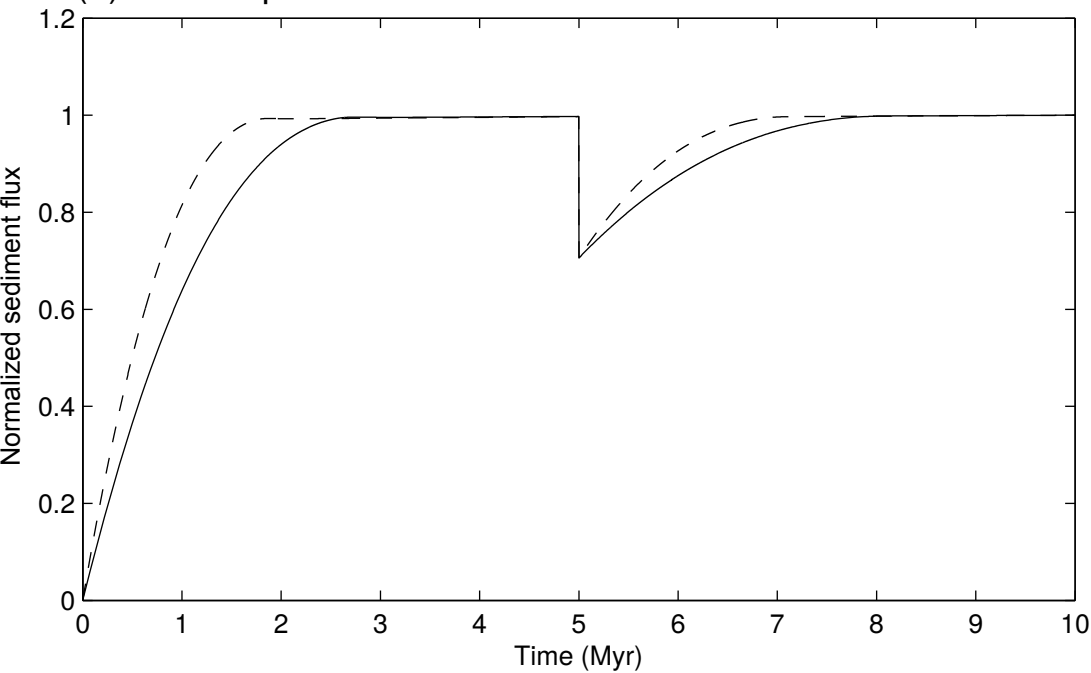
(b) Stream power model n = 1.2
