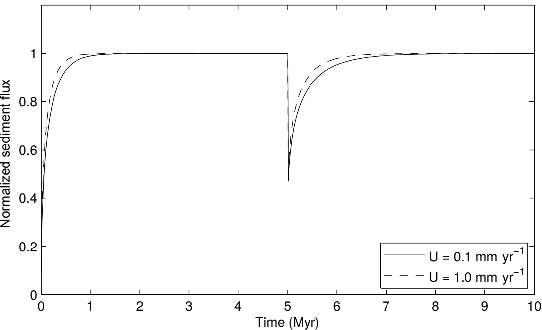
(a) Transport model \gamma = 1.2
