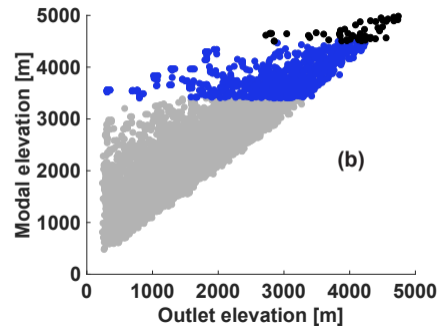
Null PH: extending through ELA
