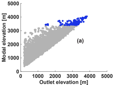
Null PH: marginal glaciation
