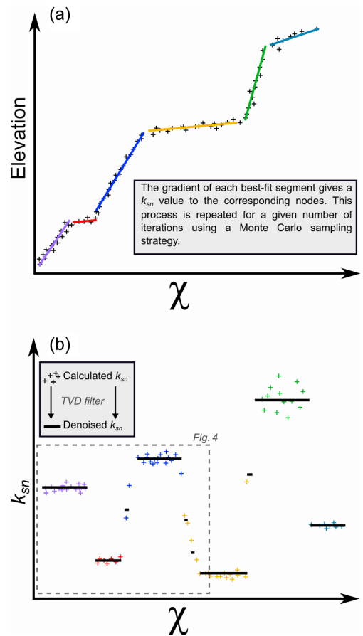
Figure 3. Extraction of normalised channel steepness ( k_{sn} ) from a river profile. (a) Example of best-fit segmentation (Mudd et al., 2014) where + symbols are individual data points and the coloured lines are the segments. (b) The associated plot of k_{sn} plotted as a function of \chi coordinate. The segmentation output results in some noise due to iterative sampling of the channel network (+ symbols). A total variation denoising filter (Condat, 2013) is then applied on the signal to extract the main variations in k_{sn} .
