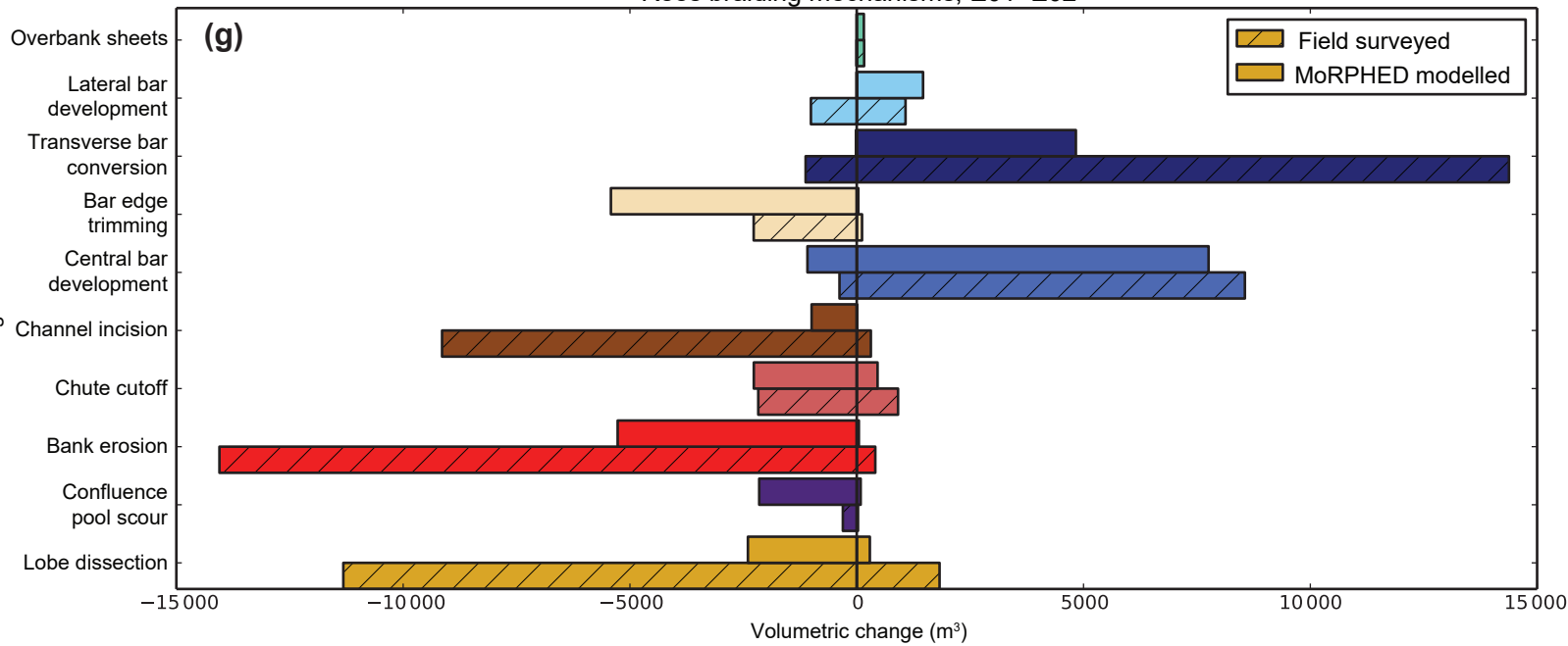
Rees braiding mechanisms, E01–E02
