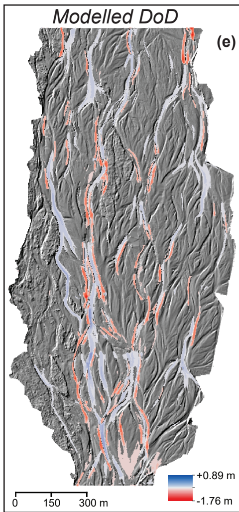
Rees braiding mechanisms, E01–E02
