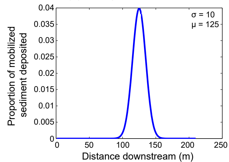
(a) Compressed Gaussian
