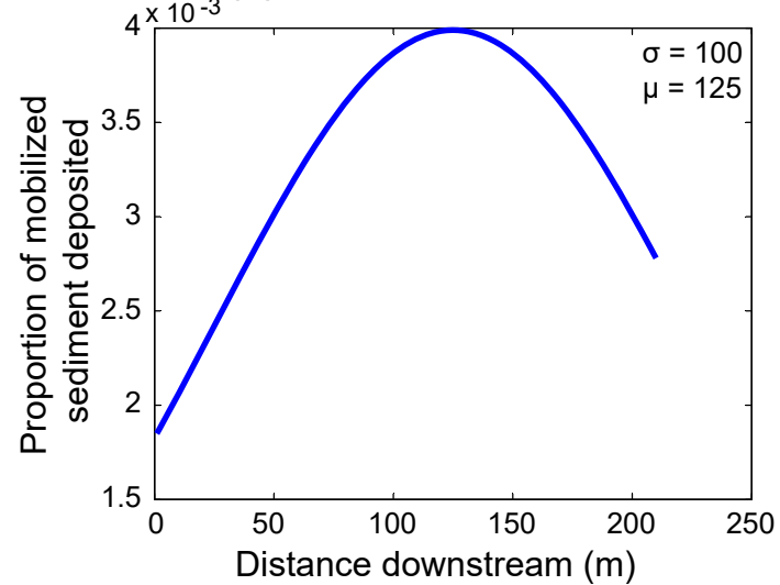
(b) Stretched Gaussian
