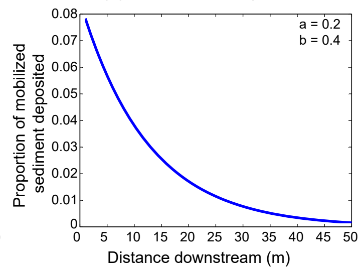
(e) Shortened exponential
