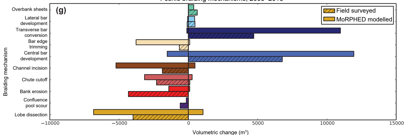
Feshie braiding mechanisms, 2003–2013
