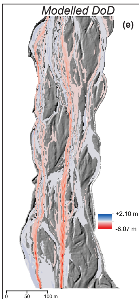
Feshie braiding mechanisms, 2003–2013
