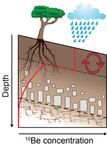
(b) Precipitation
