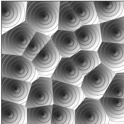
(a) Initial bedrock elevation
