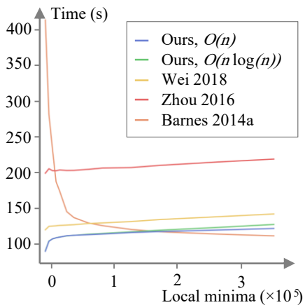
(a) Performance of algorithms
