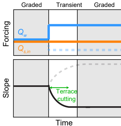
(a) Discharge ( Q_w )
