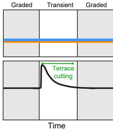
(c) Base-level fall
