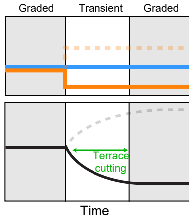
(b) Sediment supply ( Q_{s,in} )
