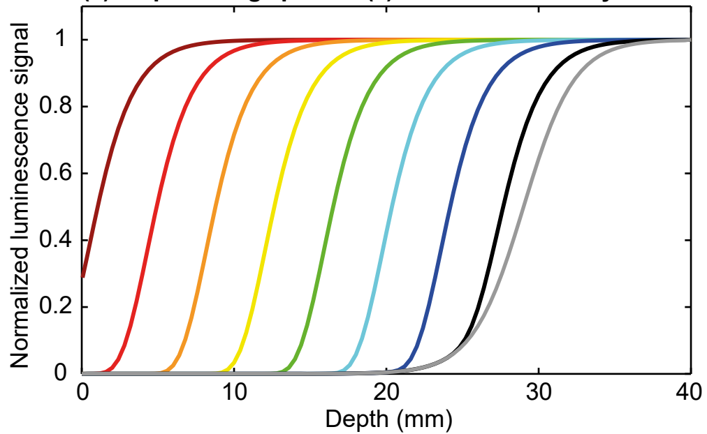
(b) Exposure age profiles (a) with \dot{D} = 2 \times 10^{-3} \text{ Gy a}^{-1}
