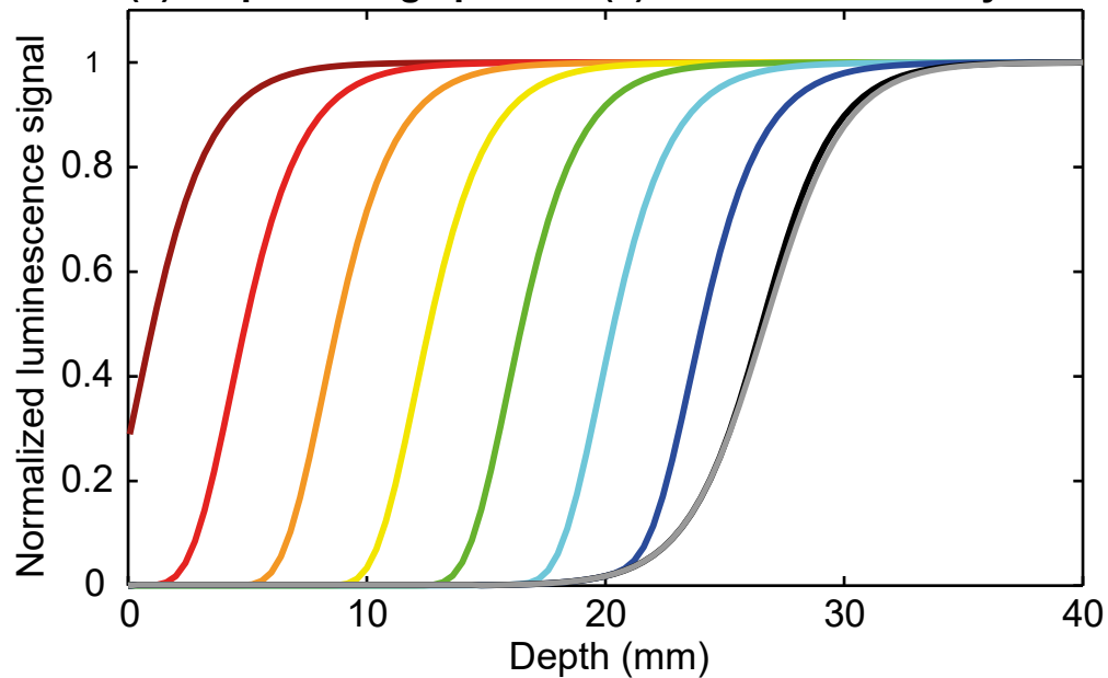
(a) Exposure age profiles (a) with \dot{D} = 8 \times 10^{-3} \text{ Gy a}^{-1}
