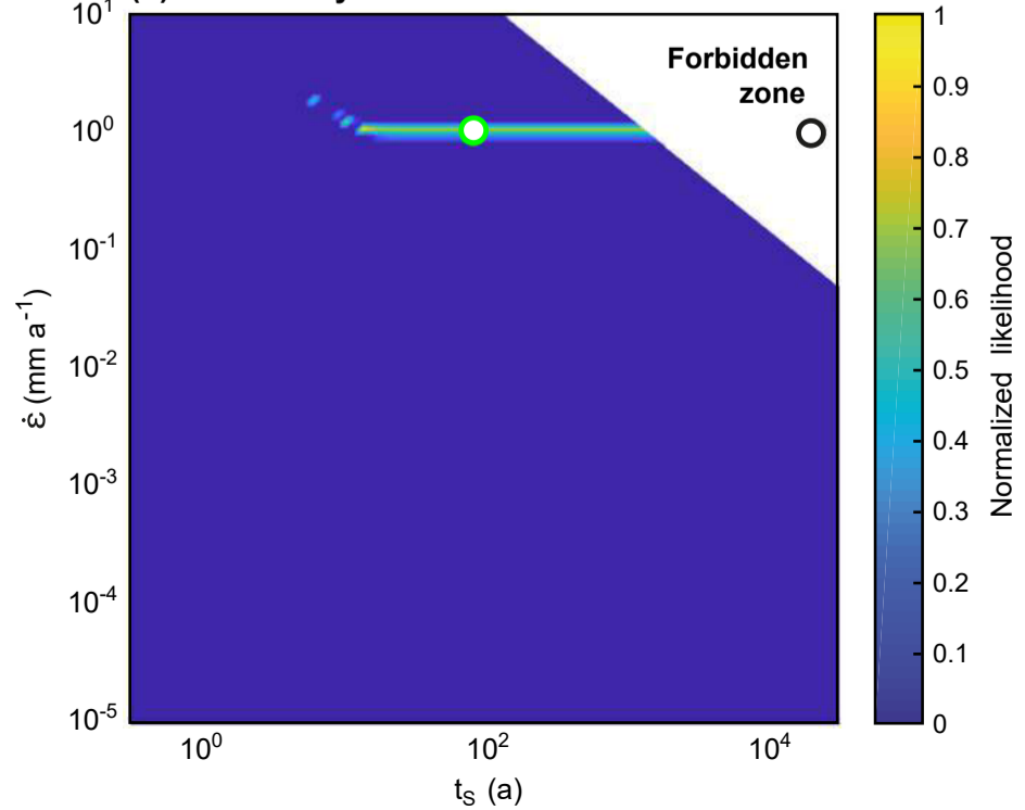
(h) Probability distribution
