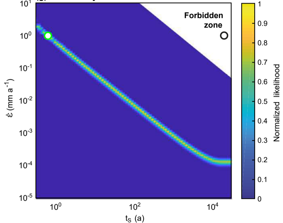
(g) Probability distribution
