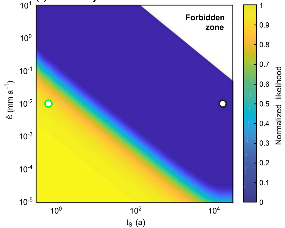
(f) Probability distribution
