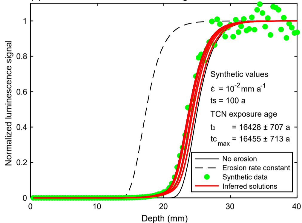
(b) Evolution of the luminescence signal
