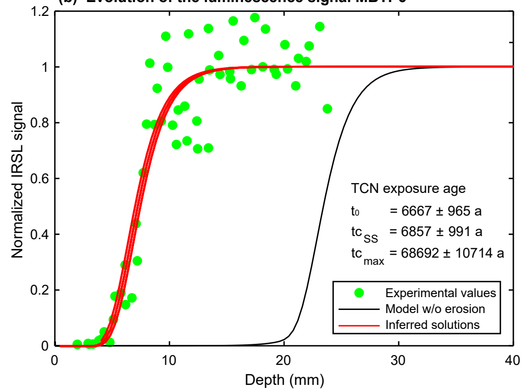
(b) Evolution of the luminescence signal MBTP6
