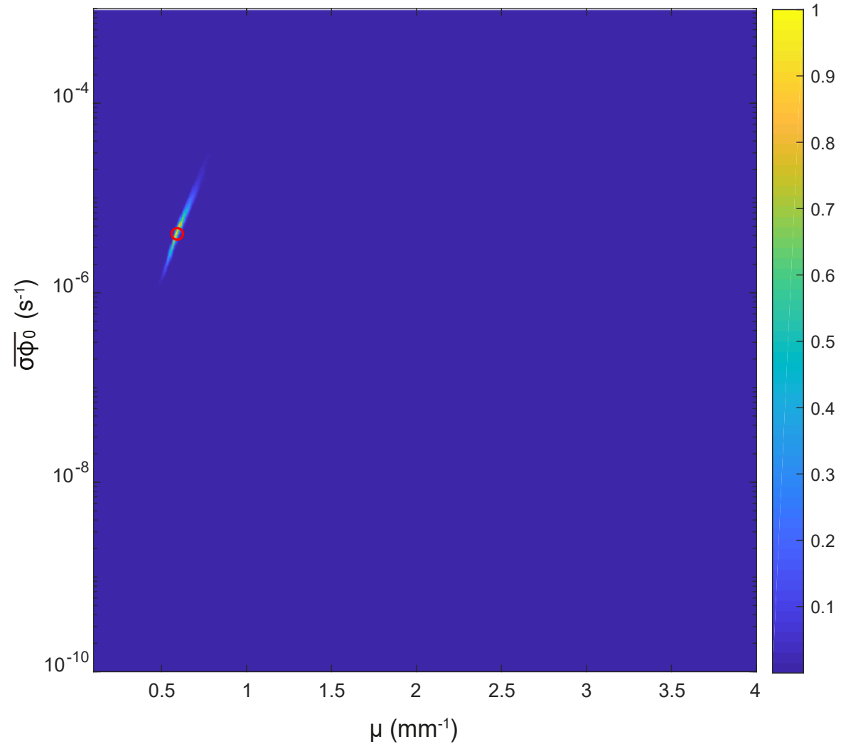
(c) Covariance of \mu and \overline{\sigma\phi_0}
