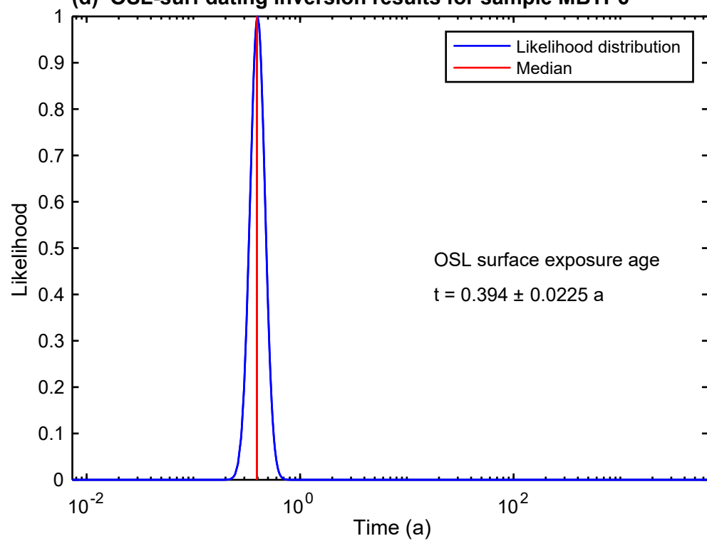
(d) OSL-surf dating inversion results for sample MBTP6
