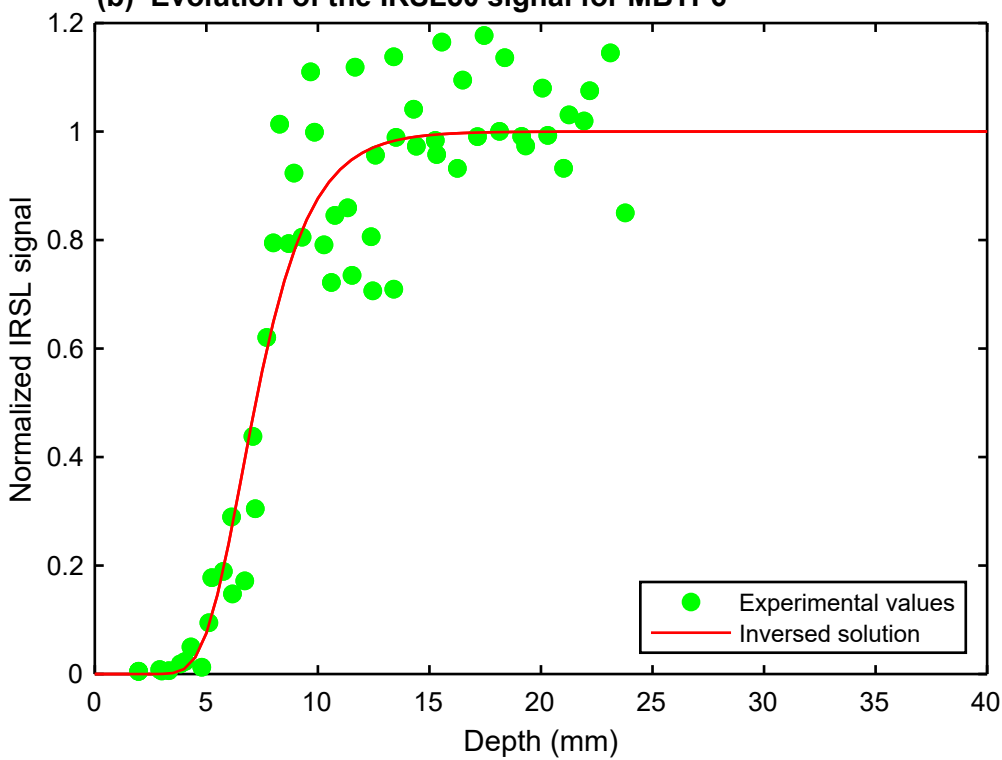
(b) Evolution of the IRSL50 signal for MBTP6
